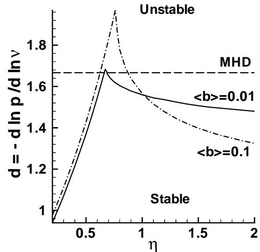
Figure 2: Exact stability boundaries for \bar{b}=0.1, 0.01 compared with the ideal MHD boundary.
