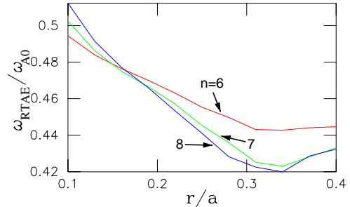
FIG. 3. RTAE frequency radial dependence for different toroidal mode numbers n = 6, 7, 8 .
