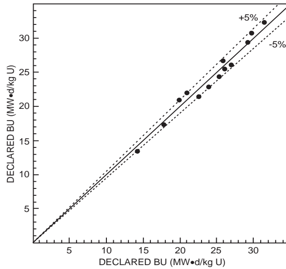
FIG. 1. Operator declared BU compared with the calculated BU values based on the 137 Cs activity measurements.
