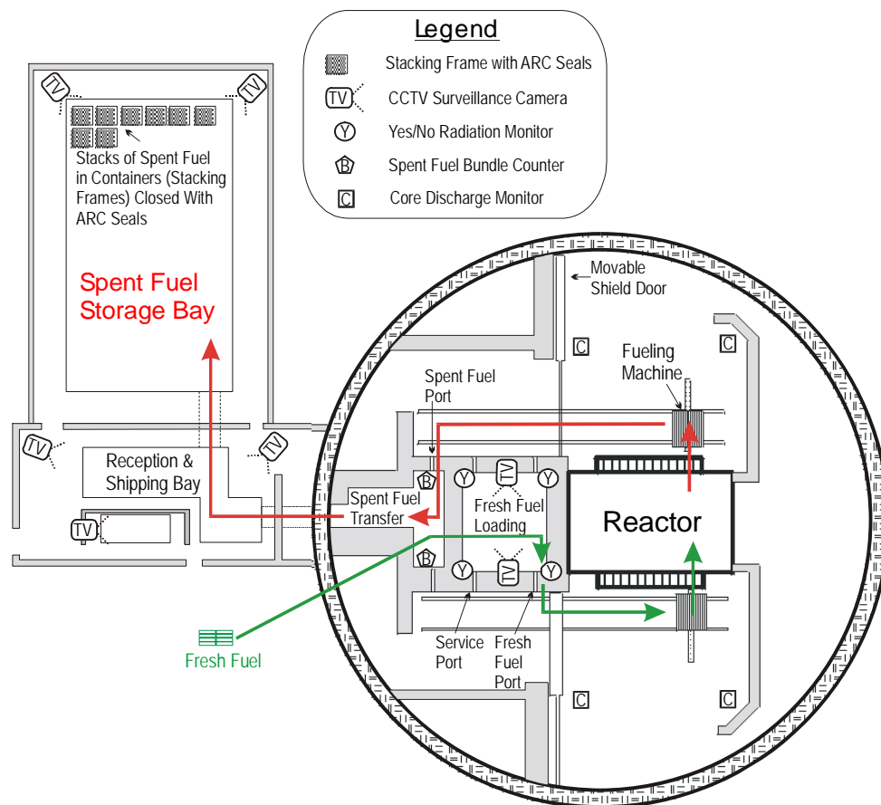
Fig. 2. Typical IAEA Safeguards Equipment for CANDU [7]
