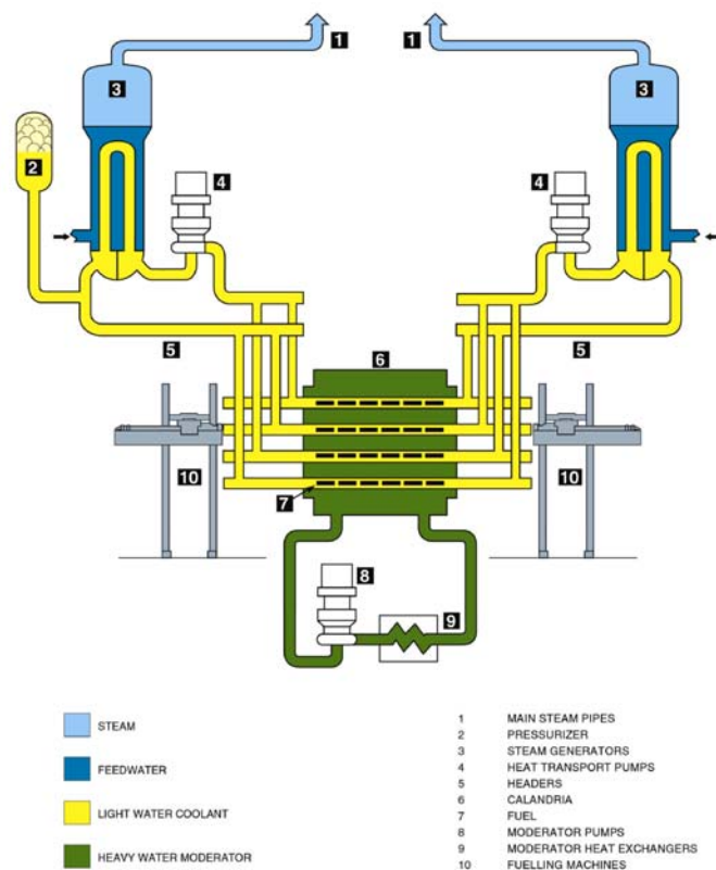
Fig. 1. Schematic of ACR-1000 Design
