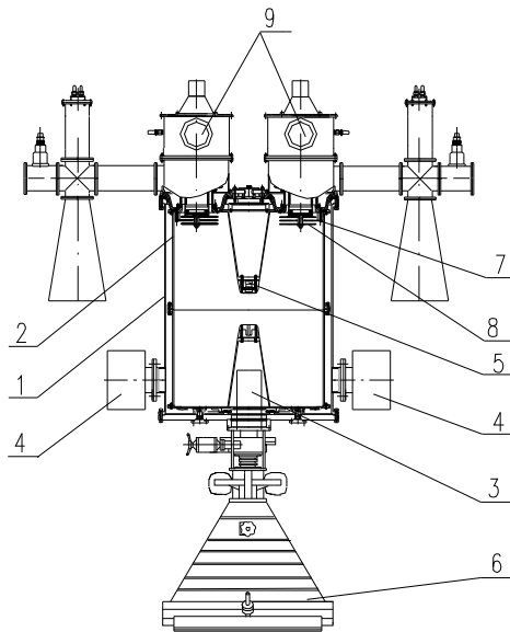
Figure 2: ILU-10 accelerator.
