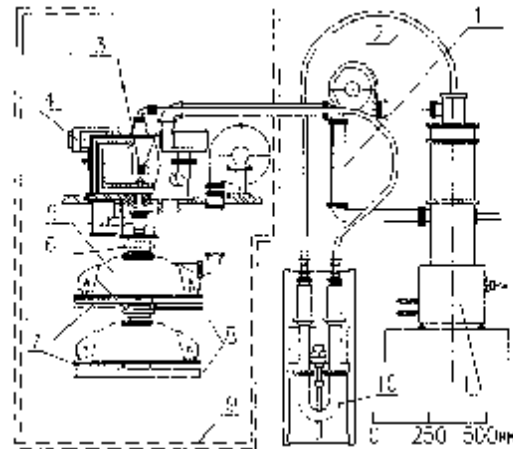
Figure 1: ILU-8 accelerator in local radiation shield.
