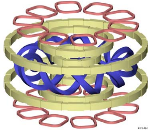
FIG. 5. Ten pairs of Resonant Magnetic Perturbation (RMP) coils (magenta).
