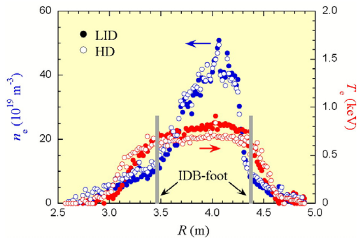
FIG. 1. Density (blue) and temperature (red) profiles of IDB-SDC plasma. Closed and open symbols represent data obtained in Local Island Divertor (LID) and Helical Divertor (HD) configurations.
