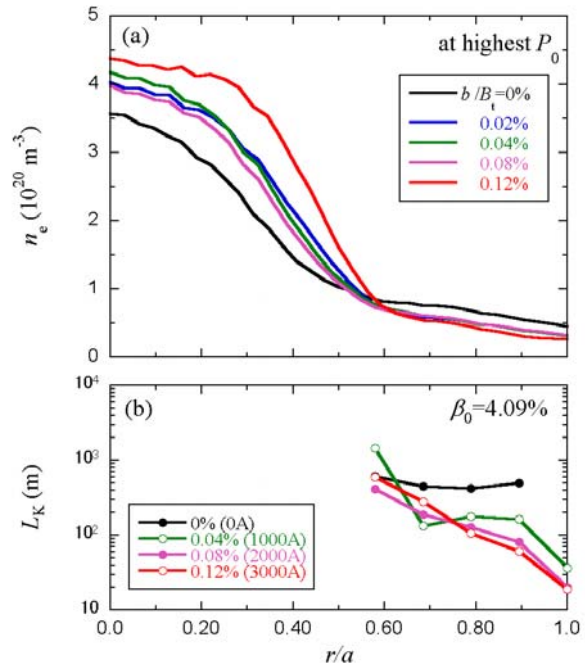
FIG. 8. Density and Kolmogorov length profiles with different RMP amplitudes.
