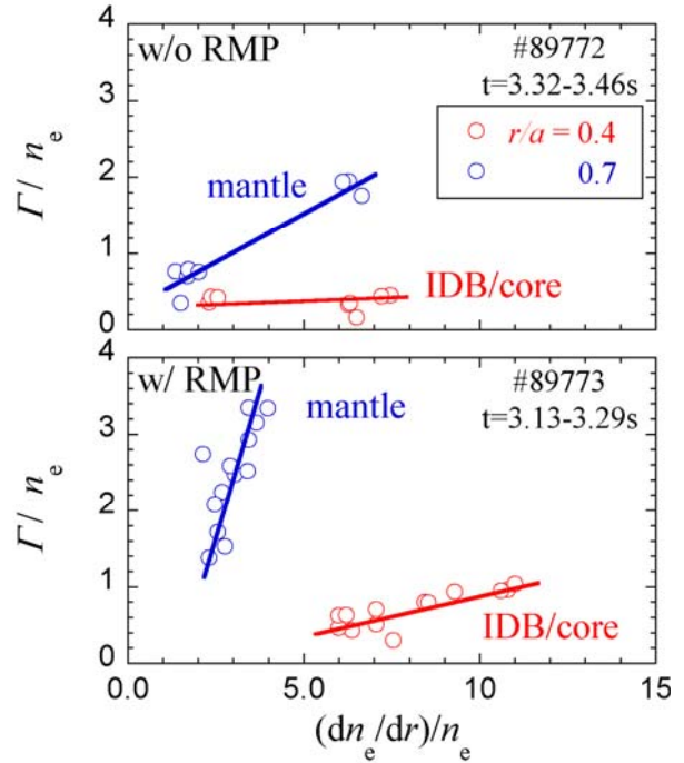
FIG. 7. Density normalized flux vs. density scale length. Gradient indicates diffusion coefficient.
