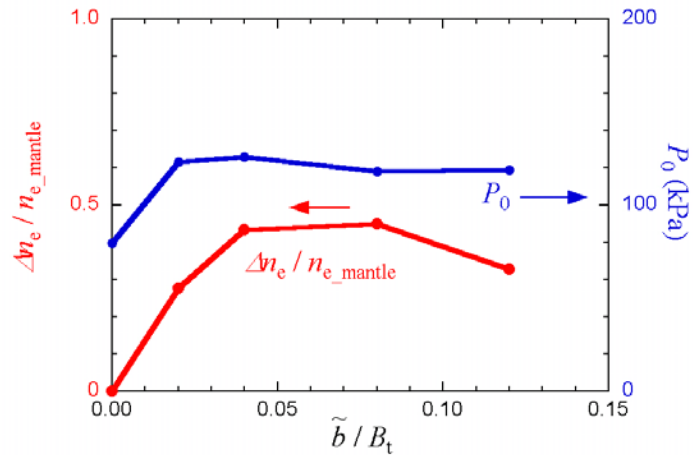
FIG. 9. Decreased mantle density \Delta n_e by RMP, depending on RMP amplitude b/B_t . \Delta n_e is normalized by n_{e\_mantle} without RMP. Central plasma pressure P_0 dependence on b/B_t is also depicted.
