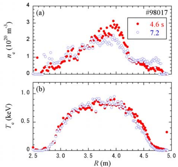
FIG. 3. Density and temperature profiles at beginning ( t = 4.6 s) and ending ( 7.2 s) of quasi-steady-state phase of IDB-SDC discharge.
