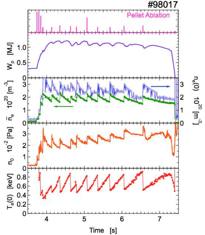
FIG. 2. Time traces of stored energy W_p , line averaged density n_e , central density n_e(0) , neutral pressure which is reflected with particle density n_0 , and temperature T_e(0) , together with injection signal of pellet (top).
