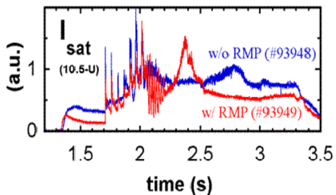
FIG. 10. Time evolution of divertor flux measured with a Langmuir probe embedded in a divertor plate.
