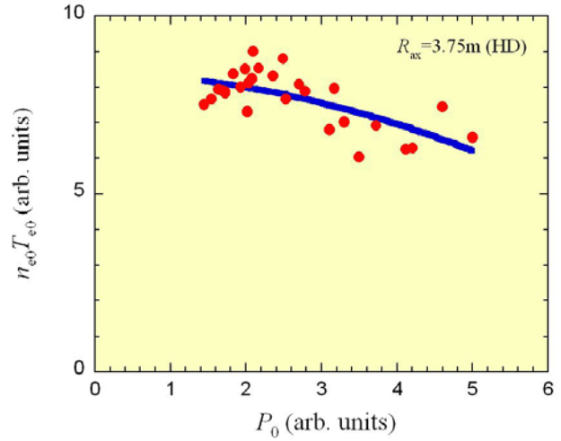
FIG. 4. Dependence of central plasma pressure n_{e0}T_{e0} on neutral pressure P_0 .
