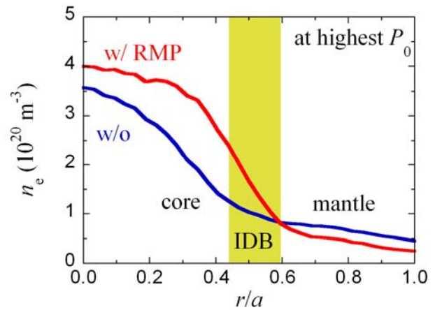
FIG. 6 Radial profiles of n_e with and without RMP.
