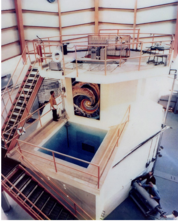
FIG. 15. TRIGA Mark II design with a bulk irradiation tank (courtesy of Kansas State University, United States of America).
