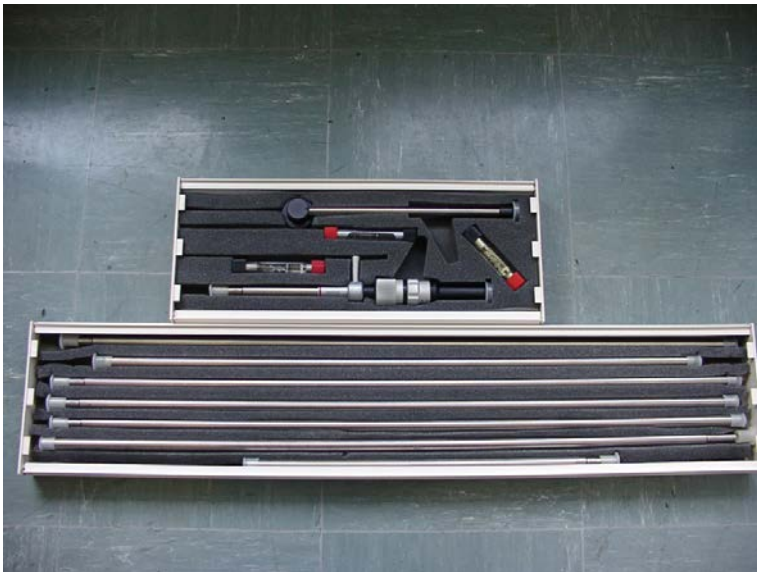
FIG. 33. Underwater endoscope (courtesy of Atominstitut, Vienna).
