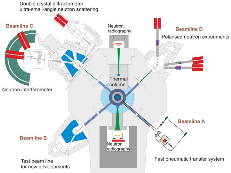
FIG. 26. Example of diverse experimental setups at the TRIGA Mark II reactor (horizontal cross-section) in Vienna, Austria (courtesy of Atominstitut, Vienna).
