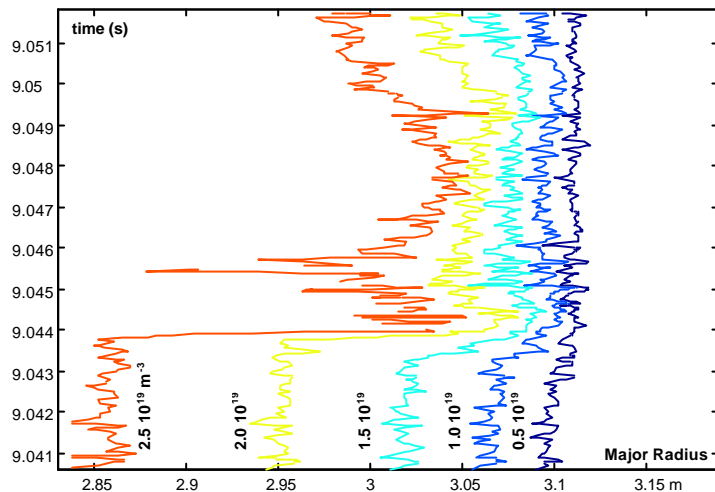
Figure 3. typical time evolution of the edge density profile during a pulsed supersonic gas injection (LFS) measured by reflectometry (TS-30510).
