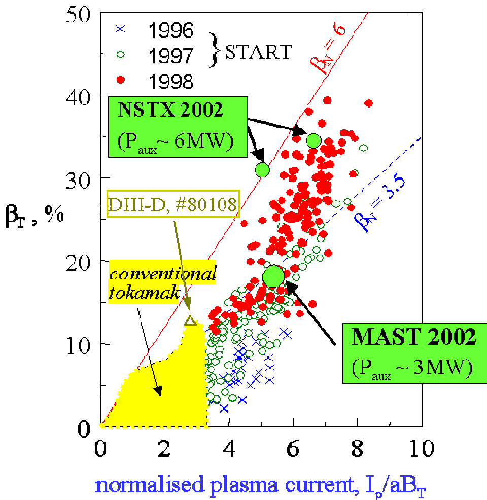
Figure 2 : \beta_T versus normalised plasma current for conventional and spherical tokamaks (courtesy A. Sykes).
