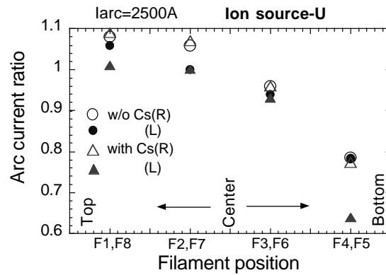
FIG 2: Arc current distribution in source
