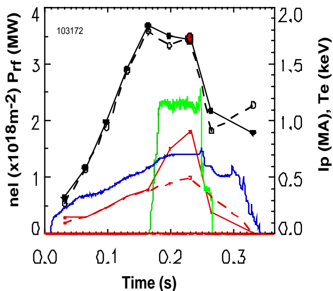
Figure 1 Time evolution of line density (black), plasma current (blue), central electron temperature (red) and rf power (green)
