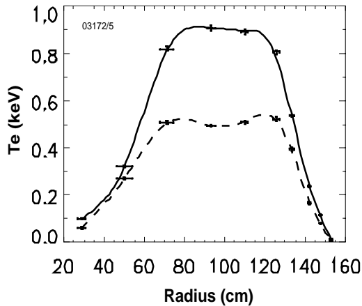
Figure 2 Electron temperature profiles at t=0.23 \text{ s} , with (solid) and without (dashed) rf
