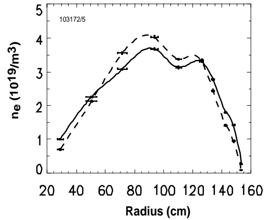
Figure 3 Electron density profiles for t=0.23 \text{ s} , with (solid) and without (dashed) rf
