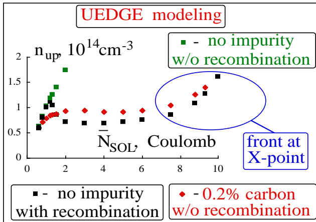
Figure 5: Tokamak Divertor Detachment Simulation
