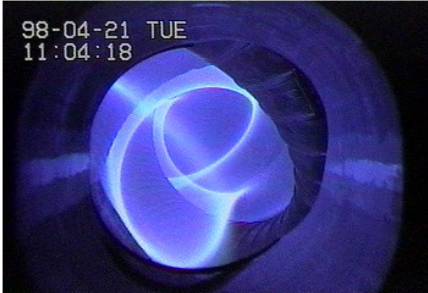
Figure 7. TV image of the LHD plasma, which is well expanded.
