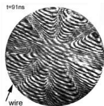
Fig 2. End-on interferogram of an 8 wire array.
