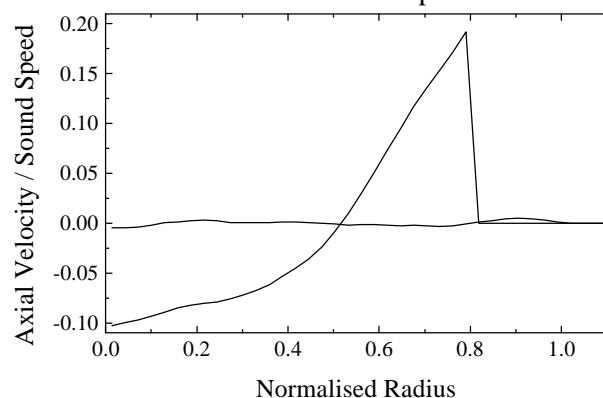
Fig. 9. Axial ion fluid velocity versus radius
