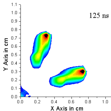
Fig 7. \rho(x,y) from a simulation of a 8 wire Al array, at 125ns.
