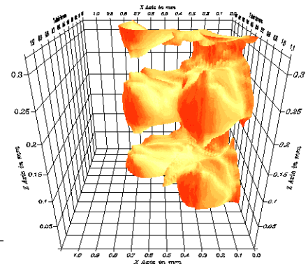
Fig 8. \rho(x,y,z) contour at 170ns from a 3D array simulation of 8 wires Al.
