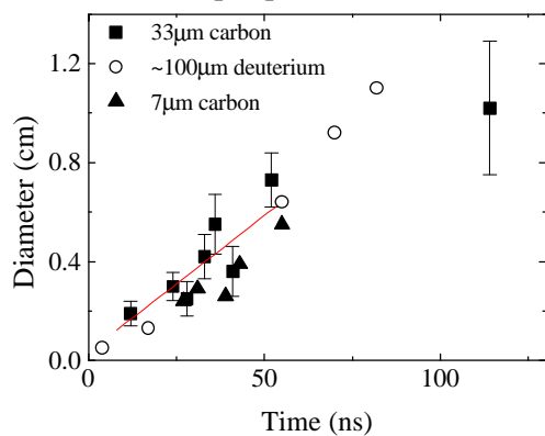
Figure 1a. Coronal plasma diameter versus time for various fibres.
