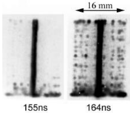
Figure 4. Gated soft X-ray images of hot-spot formation on 16 wires in an array.
