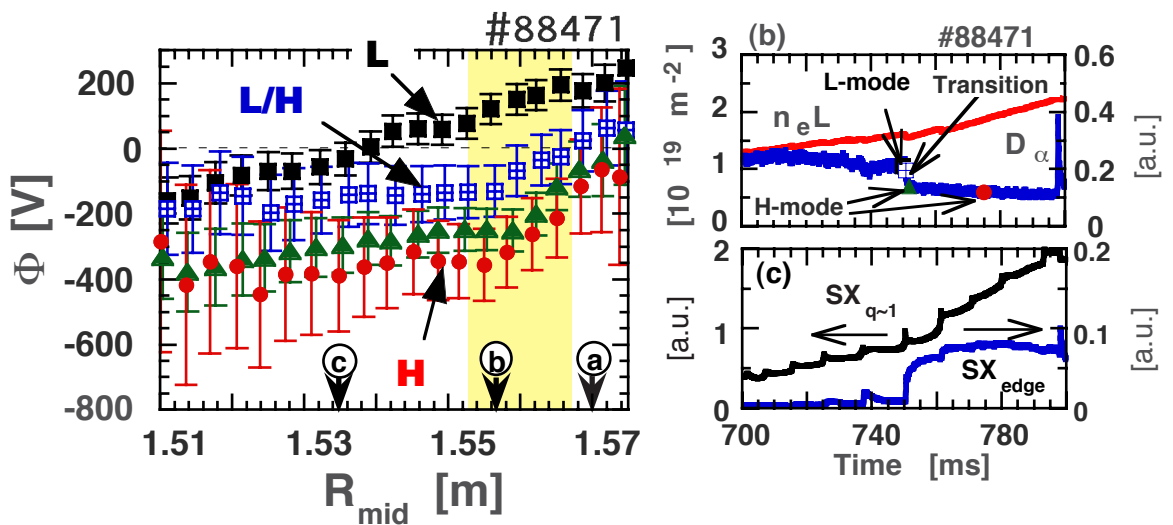
FIG.2. (a)The potential profiles near the plasma boundary. Time History of H-mode, (b)Line integrated density and D_\alpha intensity, (c)Soft X-ray intensity of around q\sim 1 and edge sight lines. Arrows in (b) on the D_\alpha trace show the time of the potential profile shown in (a). The separatrix position is estimated to be around R\sim 1.56m .
