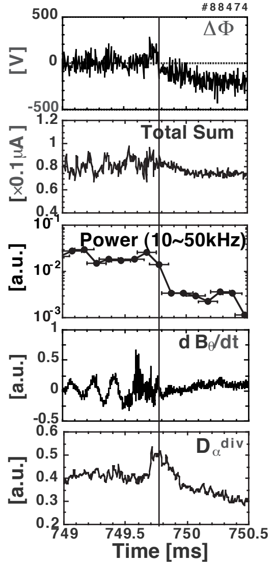
FIG.4. Fast time behaviors at the H-mode transition. The plasma potential( \Delta\Phi ), the secondary beam intensity (Total Sum), the power of the fluctuation in the beam intensity integrated from 10 to 50kHz, the magnetic probe signal of dB_{\theta}/dt and D_{\alpha} intensity when the sample volume is placed about 0.5cm inside to the plasma core compared with that shown in Fig.3(a) (shot is the same)
