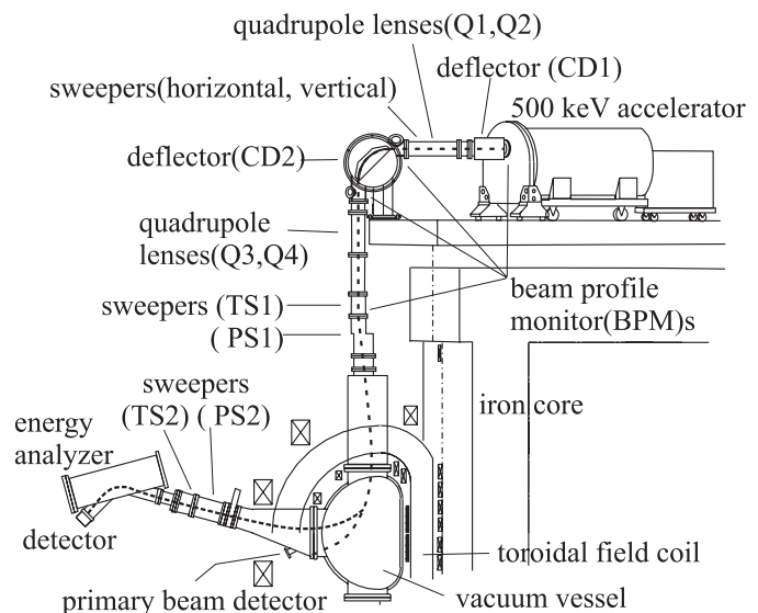
FIG. 1. Schematic View of the HIBP system on JFT-2M
