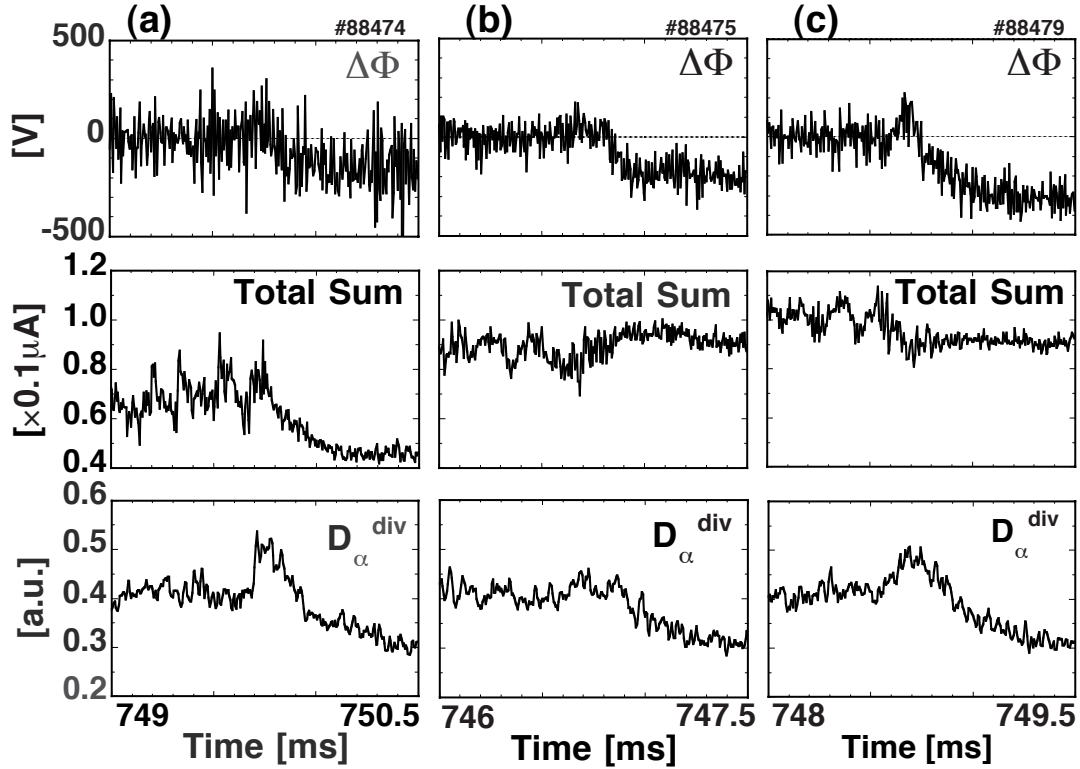
FIG.3. Fast time behaviors at the H-mode transition. The plasma potential( \Delta\Phi ), the secondary beam intensity(Total Sum) and D_\alpha intensity. The sample volume is placed about (a)1.2 cm outside the separatrix and (b)0.5 cm and (c)2.4 cm inside the separatrix. These positions are also shown in Fig.2 (a).
