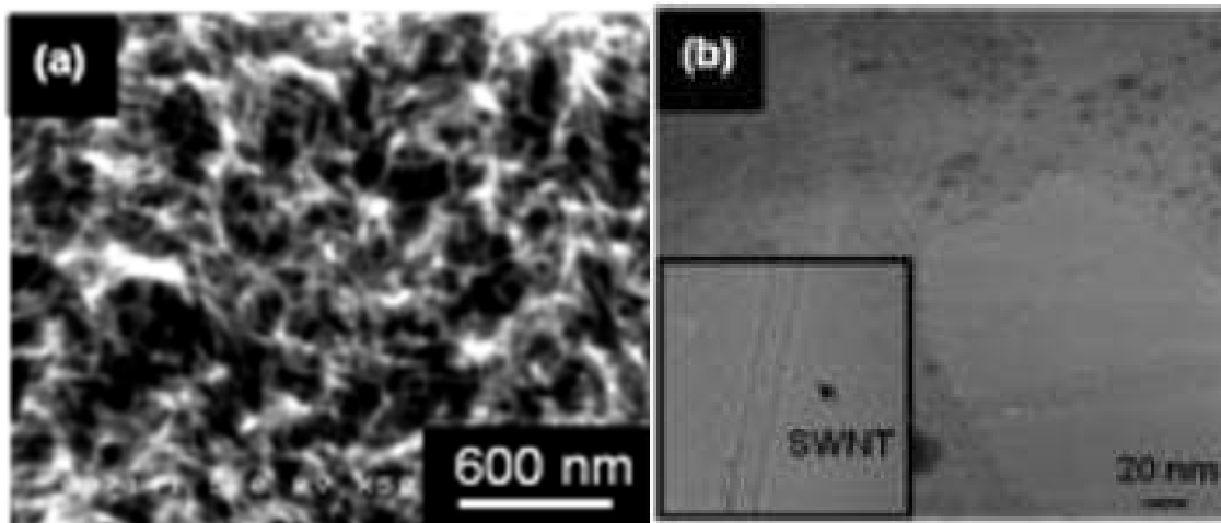
Fig. 4. Typical SEM (a) and TEM (b) images of Au catalyzed SWNTs by PCVD. Inset of (b) shows the high magnification image of individual SWNT.
