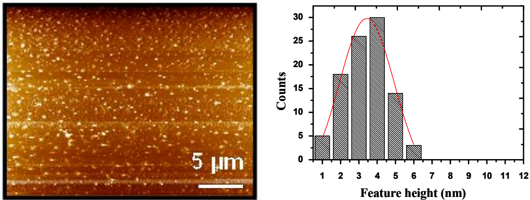
Fig. 1. AFM image and size distribution of Au nanoparticles
