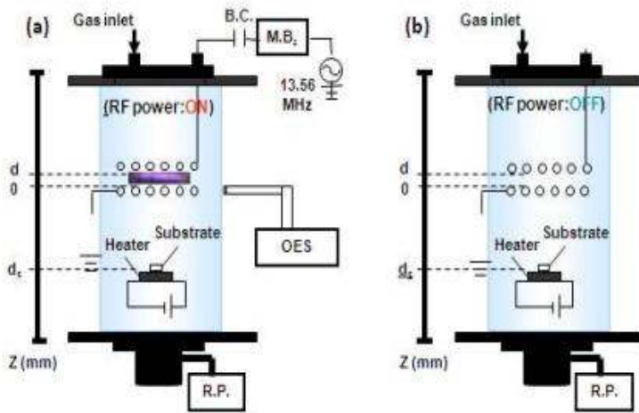
Fig. 2. Schematic diagrams of experimental setups for (a) PCVD, and (b) TCVD.
