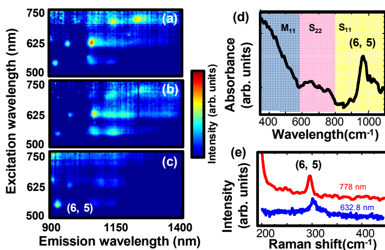
Fig. 6. (a) PLE maps of SWNTs from Au catalyst by PCVD at (a) 0-sccm, (b) 3-sccm, and (c) 7-sccm H 2 flow rates, respectively. (d) UV-vis-NIR spectrum of SDBS-dispersed SWNTs grown from Au catalyst at 7-sccm H 2 flow rate and (e) Raman spectra of SWNTs grown from Au catalyst at 7-sccm H 2 flow rate using the excitation laser wavelengths of 632.8 and 778 nm.
