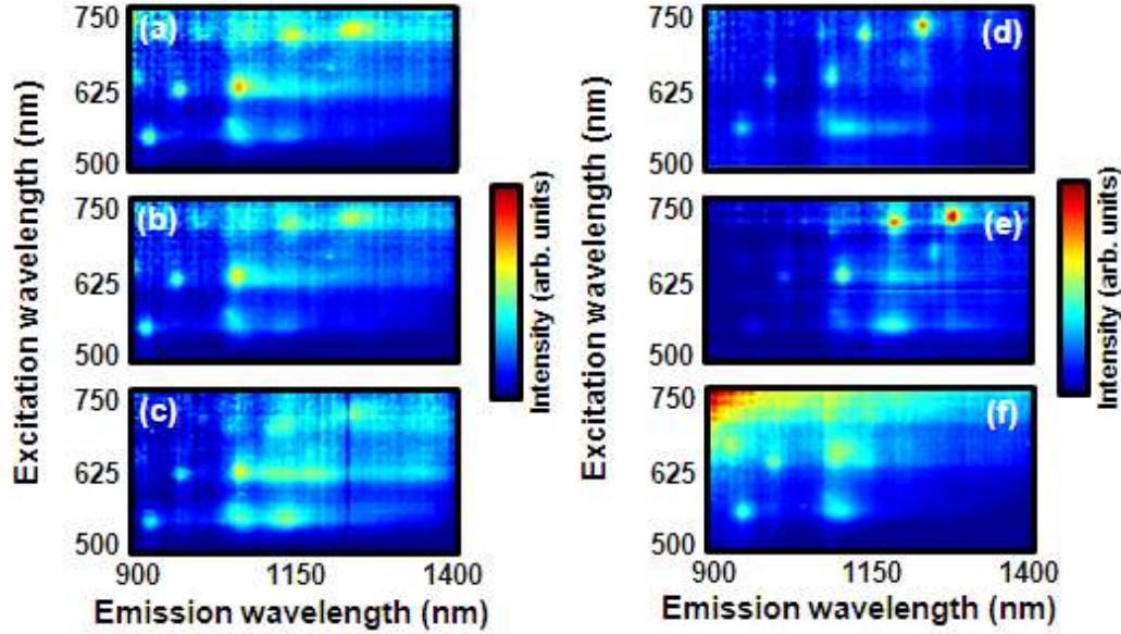
Fig. 7. PLE maps of (a-c) Fe-PCVD and (d-f) Au-TCVD SWNTs at different H 2 flow rates of (a), (d) 0 sccm, (b), (e) 3 sccm, and (c), (f) 7 sccm, respectively.
