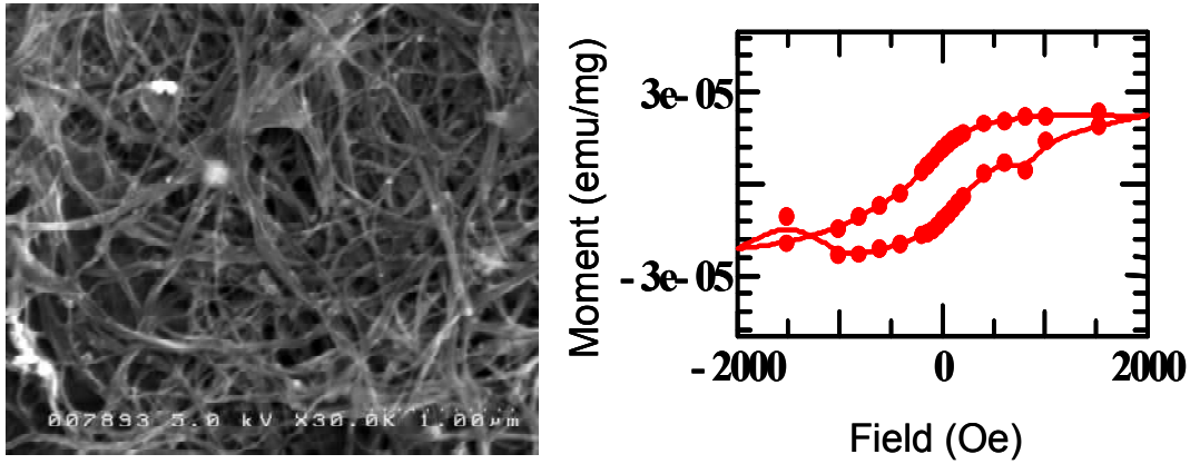
Fig. 10. (a) SEM image and (b) magnetization per mg vs applied magnetic field for the Au-PCVD SWNTs.
