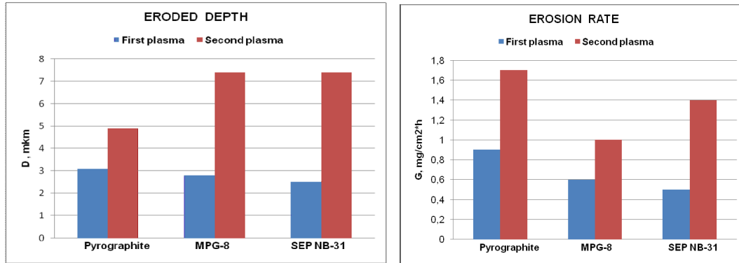
FIG 5. Erosion depth and erosion rate in double plasma experiment for 1 dpa samples of SEP NB-31, MPG-8 and pyrographite.
