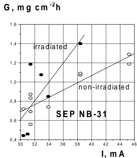
FIG. 4. Erosion rate of SEP NB-31 graphite vs plasma ion flux.
