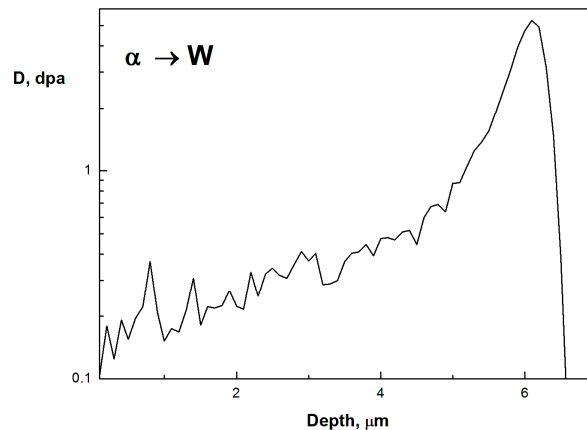
FIG. 6. Calculated profile of radiation defects produced in tungsten ( \rho = 19.35 g/cm 3 , 183.8 amu) irradiated by 4 MeV alpha-particles ( \text{He}^{+2} ) to dose = 10^{17} /cm 2 .
