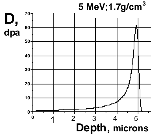
FIG. 1. Calculated profile of the primary radiation defects D (dpa) as a function of depth for a carbon material with density \rho = 1.7 \text{ g/cm}^3 after irradiation with 5 MeV carbon ions to the dose 5 \cdot 10^{17} ion/cm ^2 ( D_{\text{max}} = 65 \text{ dpa} lies at \sim 5 \mu\text{m} , \langle D \rangle = 9.7 \text{ dpa} ).
