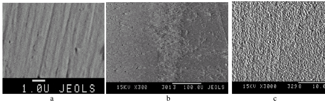
FIG. 7. Tungsten surface modification by high-energy \alpha -particles; a) the surface as prepared, b) the border of irradiation area on tungsten sample with the received ion fluence 10^{18} ion/cm 2 : the left part was not irradiated; c) as irradiated with ^4\text{He}^{+2} ions to fluence 3 \cdot 10^{18} ion/cm 2 (scale bars in microns).
