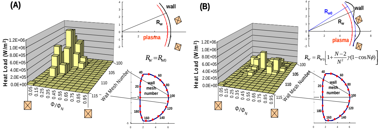
Fig.6 Two dimensional heat loads on an axis-symmetric and axis-asymmetric first wall for F_{exp}=1.2 and R_{sift}=0 with ferrite plates.
