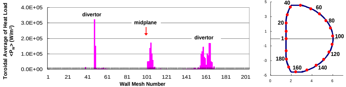
Fig.5 Typical poloidal distribution (toroidal average) of heat load on the first wall
