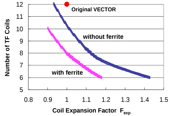
Fig.9 Contours of number of TF coils and coil expansion factor to meet peak heat load of 1\text{MW/m}^2 with and without ferrite plates ( \Delta R_{p-F}=0.63\text{m} , \Delta T_F=0.25\text{m} )
