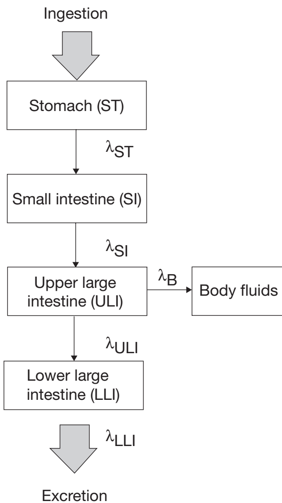
FIG. 3. Mathematical model used to describe the kinetics of radionuclides in the GI tract (reproduced from Ref. [14]).
