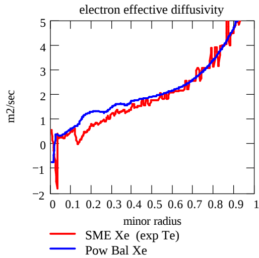
FIG. 5. Effective diffusivity TS 30007 (see text)
