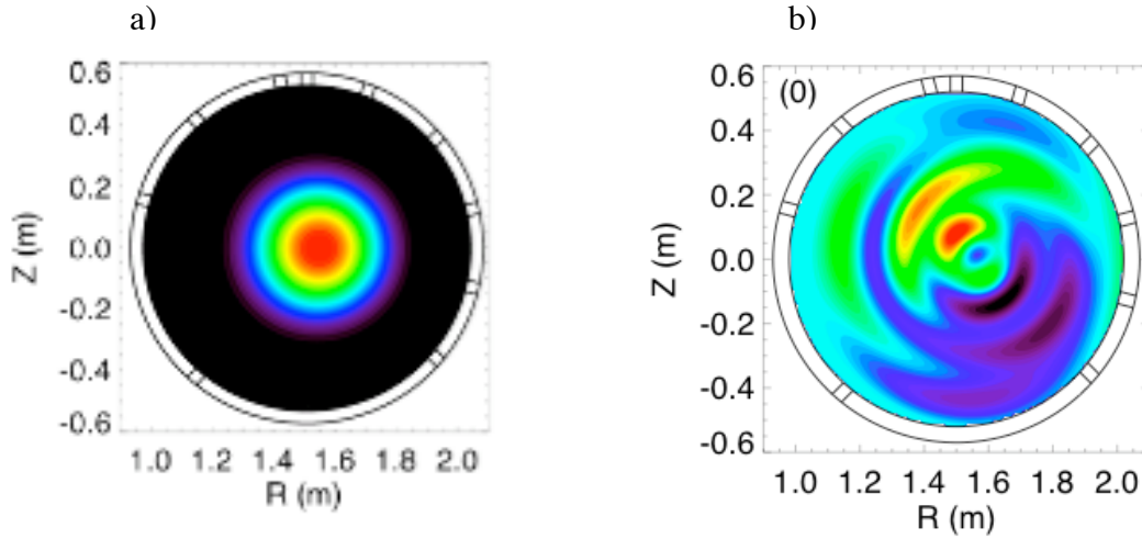
FIG. 7. Contours of constant soft x-ray emissivity, in the poloidal plane, for (a) standard and (b) PPCD plasmas. For (b) the mean signal is subtracted, so that the fluctuating islands are visible (red islands indicate a positive value and blue a negative value, relative to the mean).
