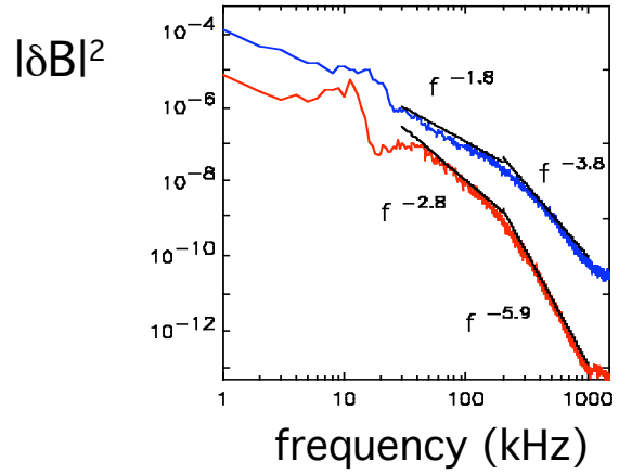
FIG. 8. Frequency spectrum of magnetic fluctuations for standard plasmas (top curve) and PPCD plasmas (bottom curve). The straight lines, described by the power laws shown, are fits to the data.
