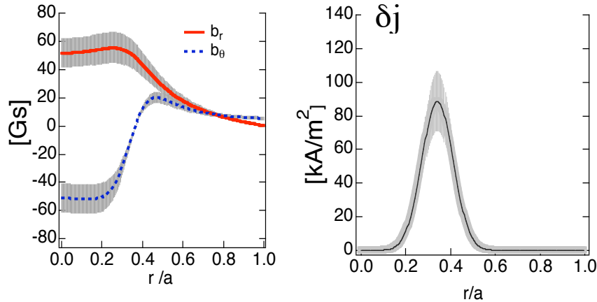
FIG. 1. Radial profiles of radial and poloidal magnetic fluctuations (left figure) and toroidal current density fluctuations (right figure). The fluctuations are obtained from inversion of laser Faraday rotation data. The current measurement assumes a Gaussian profile for the inversion.
