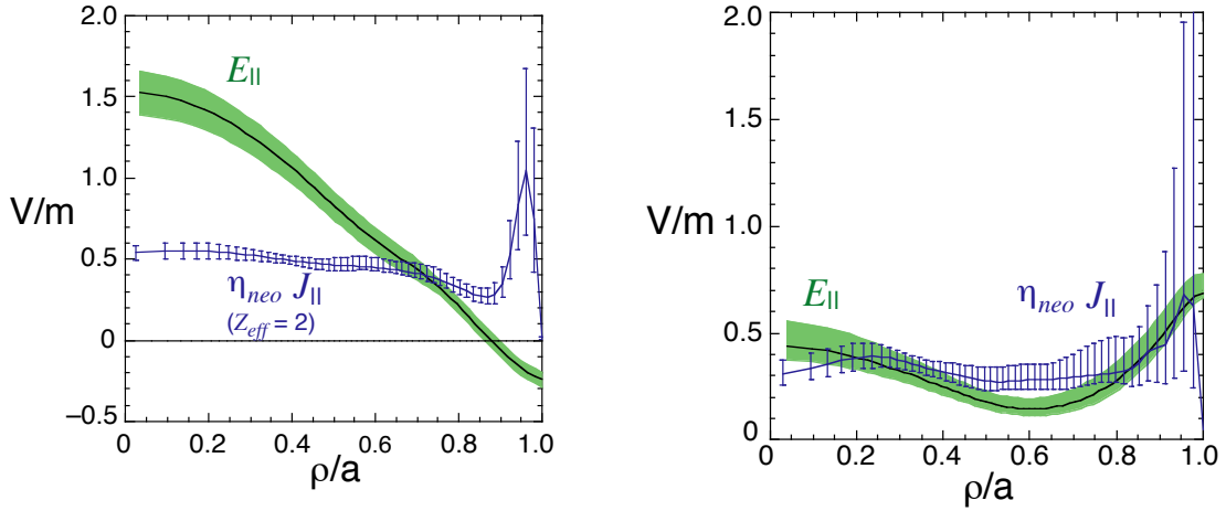
FIG. 6. Radial profile of mean electric field and current density terms in Ohm's law for (a) standard plasmas and (b) PPCD plasmas. The difference between the two curves indicates the dynamo effect.
