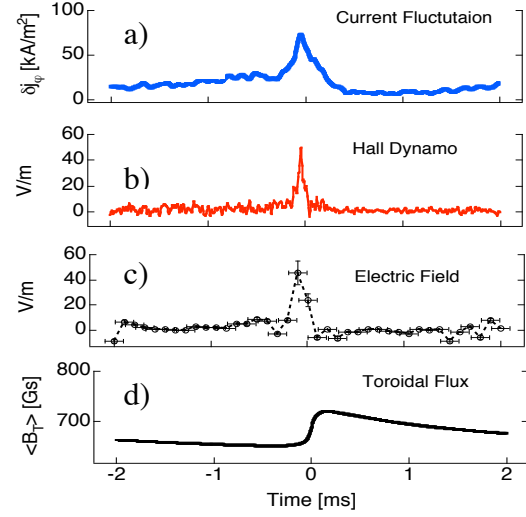
FIG. 2. (a) Toroidal current density fluctuations, (b) Hall dynamo \langle \delta \mathbf{j} \times \delta \mathbf{B} \rangle_{\parallel} / ne , (c) parallel mean electric field, and (d) toroidal magnetic flux vs time through a sawtooth cycle.
