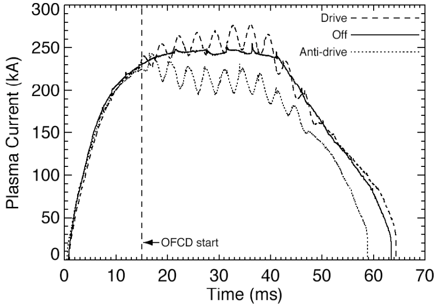
FIG. 9. Plasmas current vs time for three cases: oscillating field current drive (OFCD) with toroidal and poloidal loop voltages relative phases set for maximum helicity injection (dashed curve), OFCD with voltages phases set for maximum helicity removal, and OFCD off.
