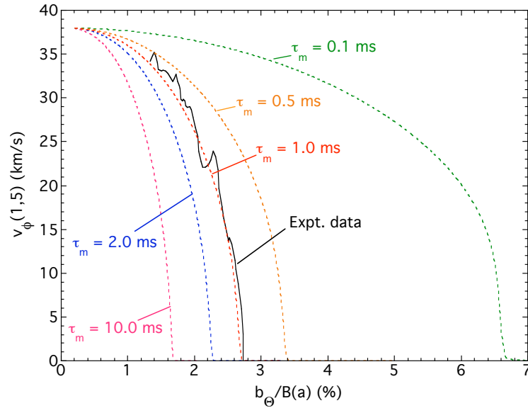
FIG. 5 Trajectory of toroidal velocity vs poloidal magnetic fluctuation amplitude for the m = 1 , n = 5 mode (solid line), as the mode rotation decreases, and theoretical predictions for trajectory, based on torques from shell eddy current, for different values of the momentum confinement time, \tau_m .
