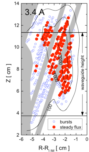
Fig. 13: 2D structure of the suprathermal electrons, measured by RFA
