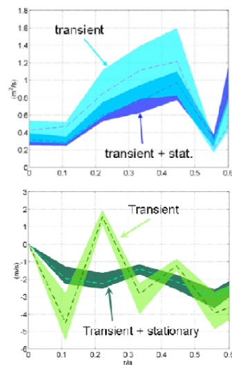
Fig. 12: Nitrogen D (top) and V (bottom) profiles, from by purely transient method and transient +stationary method)
