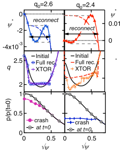
Fig. 14: Off-axis and global crash associated to the full reconnection of the Double-Tearing Mode. Reconstructed experimental profiles and XTOR simulations.
