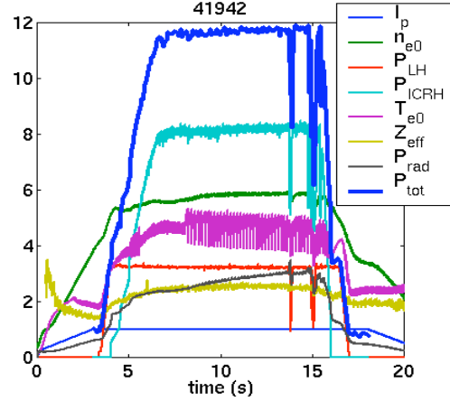
Fig. 7: time history of a 12 MW discharge, obtained after PFC cleaning. Powers are in MW, current in MA, density in 10^{19} \text{ m}^{-3} , temperature in keV.
