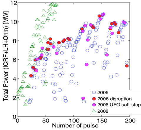
Fig. 6: Total additional power vs number of pulses realised for a power increase phase in 2006 (circles) and in 2008 (triangles).
