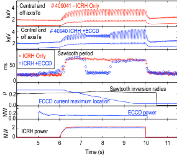
Fig. 8: Comparison of two consecutive shots – one with 2.3MW of ICRH and no ECCD and one with ECCD added.
