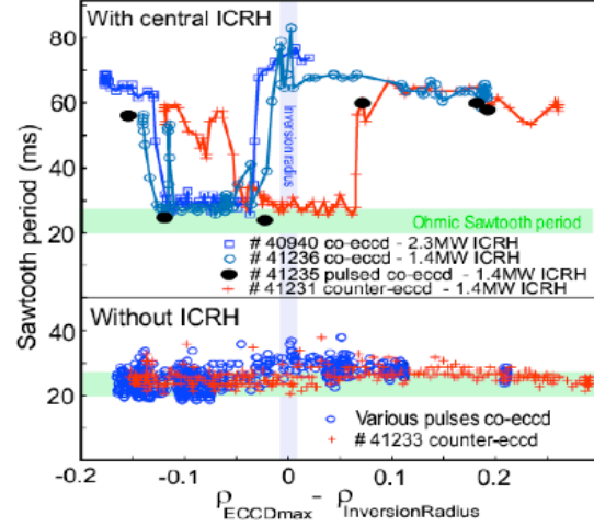
Fig. 9: Sawtooth period versus distance between ECCD location and the inversion radius for co- and counter-ECCD. a) and b) shows the result with and without central ICRH
