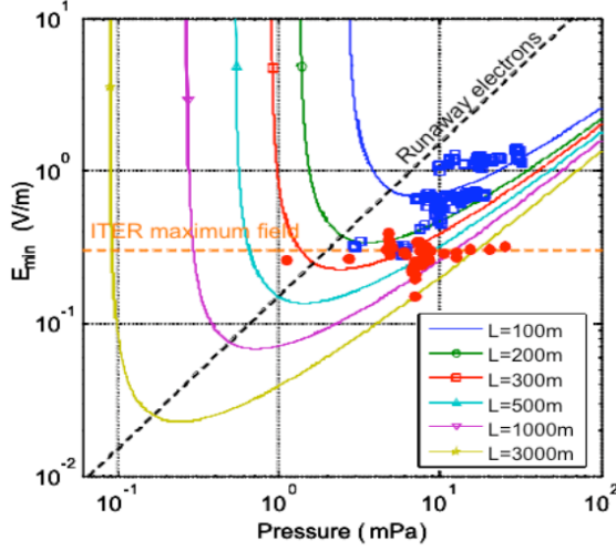
Fig. 10: applied electric field vs pre-fill pressure for a number of successful start-up attempts, both with and without ECRH assistance. Open squares correspond to ohmic startup, full circles to ECRH assisted startup. L is the toroidal connection length. Townsend curves are also shown.
