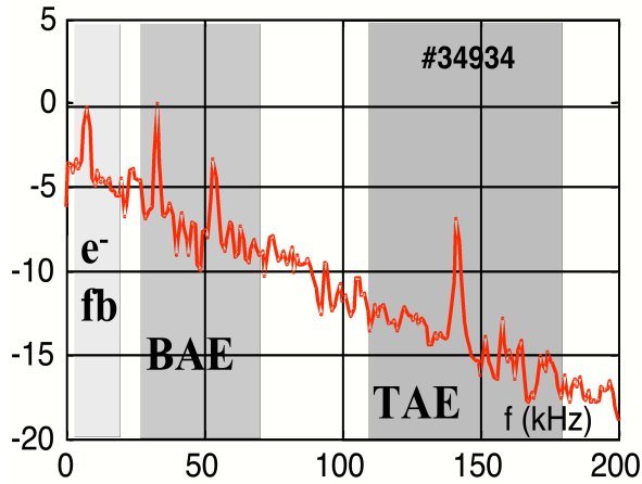
Fig. 16: Example of high frequency modes spectrum observed with reflectometry ( r/a \sim 0.3 ) in a LH+ICRH discharge.
