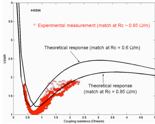
Fig. 1: Shot 40596: VSWR as a function of the coupling resistance: experimental data from a single discharges (symbol: +); electrical simulation (bold lines).
