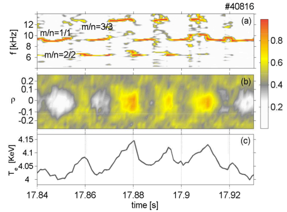
Fig. 17: (a) Spectrogram of detected modes. (b) 2D-surface representing the evolution of the electron temperature T_e - \langle T_e \rangle . (c) Central electron temperature time trace
