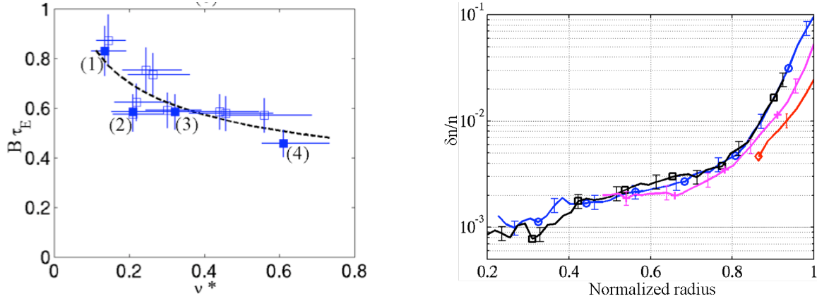
Fig. 11: Left: energy confinement time behaviour vs collisionality. Right: radial profiles of density fluctuations \delta n/n for discharges with different \nu^* (diamonds: \nu^* \sim 0.13 ; plus: \nu^* \sim 0.20 ; circles: \nu^* \sim 0.32 , squares: \nu^* \sim 0.61 , labeled as 1,2,3,4 in the left panel).
