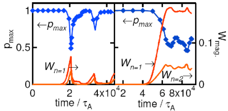
Fig. 15: Non-linear simulation of q=2 sawtooth regime and (2,1) mode saturation with XTOR
