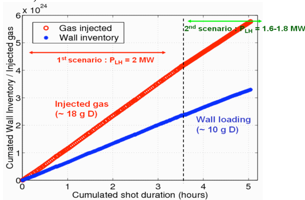
Fig. 4: Injected gas and wall D inventory vs cumulated discharge duration for the dedicated campaign.
