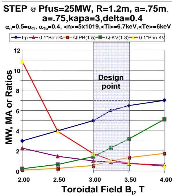
Fig.2. Results of the system code analysis. The design point for P_{fus}=25MW , R=1.2m , a=0.75m , \kappa=3 , \delta=0.4 and H=1.5 (IPB98) is shown with a shaded area.
