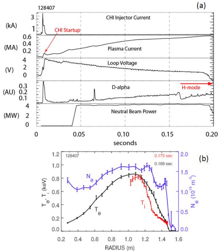
Fig 2: (a) Traces from a CHI started discharge that was coupled to induction using the central solenoid. Shown are the CHI injector current, the CHI produced plasma current, the pre-programmed loop voltage, the divertor D_\alpha signal and the applied neutral beam power. Note the steepening in the edge density gradient during the H-mode phase. (b) Shown are the electron temperature and density profiles from a Thomson scattering diagnostics soon after transition to H-mode and the ion temperature profile from a CHERS diagnostic.
