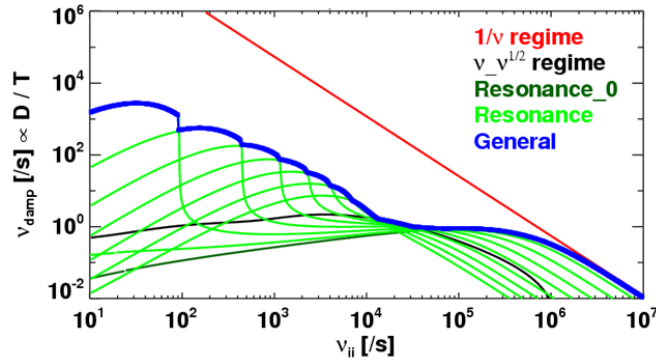
Fig.3 Rotational damping rates as a function of ion-ion collision frequency evaluated by each formula in 1/\nu regime [8], \nu_{\nu^{1/2}} regime [21], and general formula including each resonance ( \ell = 0 , Resonance_0 and \ell > 0 , Resonance) [14]. Parameters are R_0 = 2m , \varepsilon = 0.3 , q = 2.2 , n_e = 5 \times 10^{19} m^{-3} , \omega_E / 2\pi = f_\phi = 10^4 , n = 3 , and \delta_{mn} = 10^{-3} e^{-(m-5)^2/50} .
