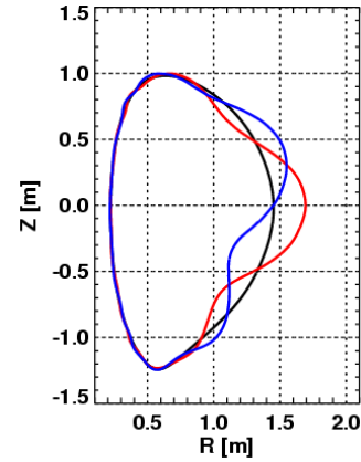
Fig.2 The most sensitive external field on the plasma boundary,
