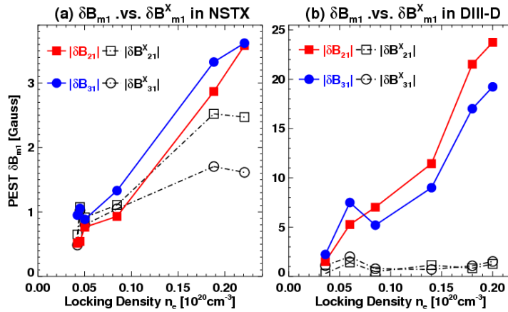
Fig.1 Comparison between \delta B_{mn} and \delta B_{mn}^x at the rational surfaces as functions of critical density in (a) NSTX (b) DIII-D locking experiments.
