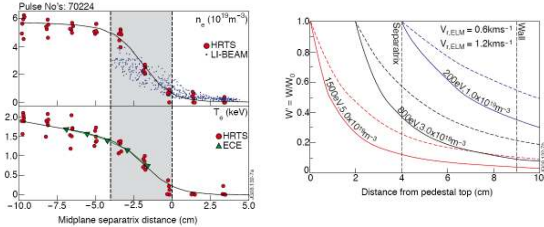
Figure 3: (a) Inter-ELM pedestal profiles. Solid lines are tanh fits to the HRTS data. (b) Model predictions for W'(r) for different initial filament positions (initial n_e , T_e at launch are marked) and radial velocities (solid line = 600 m/s, dashed line = 1200 m/s); these results should be compared with a measured value at the wall of 8.8%. Reproduced from [Pitts08].
