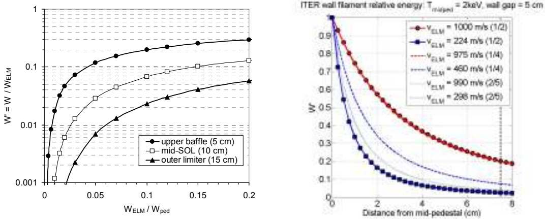
Figure 4: (left) Predicted fraction of ELM energy reaching the wall in ITER, W' , as a function of ELM energy, based on extrapolation from JET using equations (2) and (8), at three radial locations (the upper baffle, in mid-SOL and at the outer limiter); (right) similar prediction for W' at the upper baffle using the parallel loss model for natural (20 MJ, \Delta W/W_{ped} \sim 13.3\% ) and mitigated (1 MJ, \Delta W/W_{ped} \sim 0.66\% ) ELMs; the velocities were obtained using equation (9) with \alpha = 0.5 (solid lines), \alpha = 0.4 (dotted lines) and \alpha = 0.25 (dashed lines); the three lines are virtually identical for the natural ELM and yield W' \sim 25\% , while for the mitigated ELM \alpha = 0.5 , 0.4 and 0.25 give W' \sim 7.5\% , 4\% and 2.5\% , respectively.
