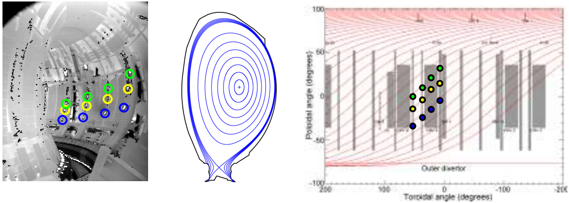
Figure 1: IR image during a Type-I ELM (left), pre-ELM magnetic equilibrium (middle) and ELM-filament footprint and pre-ELM magnetic field (right)[Jakubowski08].
