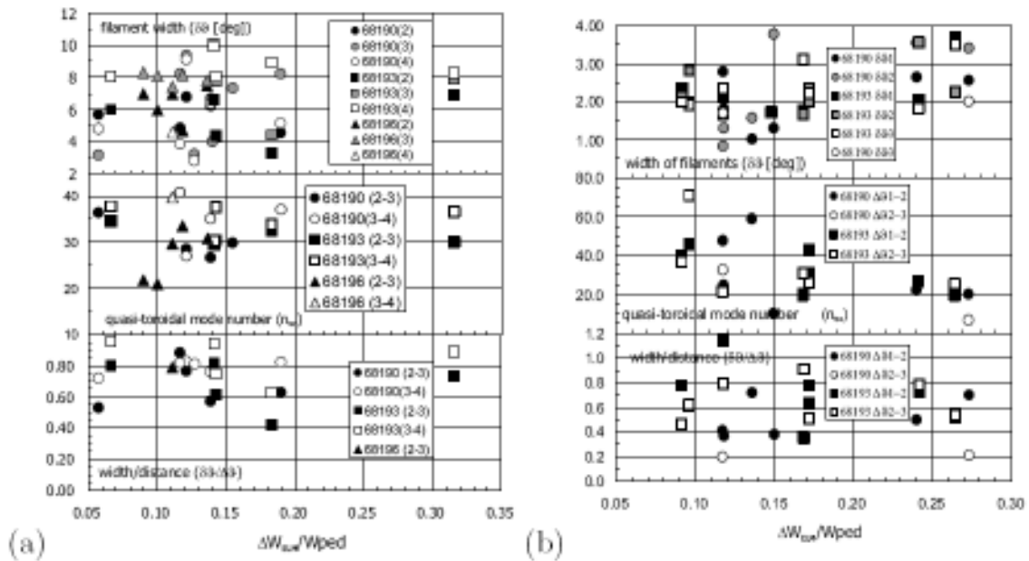
Figure 2: Variation of filament footprints structure with ELM size for the outer limiters (a) and upper dump plates (b): top - footprint width, middle - toroidal mode number at the wall radius, n_w , bottom - fraction of the filament imprint width to the separation of the filaments. Reproduced from [Jakubowski08].
