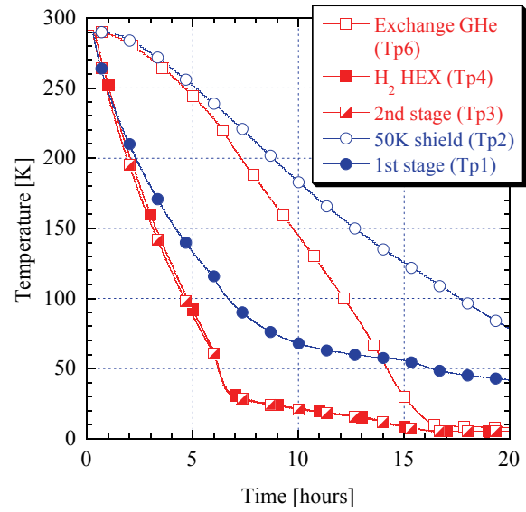
FIG. 7. Cool-down curve.
