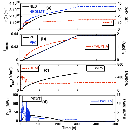
FIG. 4. Temporal evolution of plasma parameters with the pre-programming power of P_{EXT-pre}=25 MW and \tau_{rise}=300 sec.
