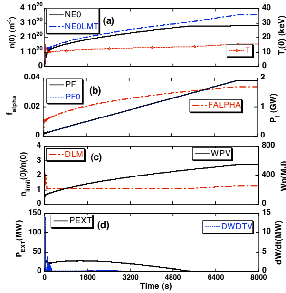
FIG.5. Temporal evolution of plasma parameters with the pre-programming power of P_{EXT-pre}=25 MW a long fusion power rise-up time of \tau_{rise}=7200 sec.
