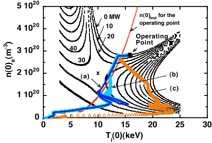
FIG.6. Three operation paths to ignition point on POPCON diagram for (a) \tau_{rise}=2 hours and P_{EXT-pre}=25 MW (corresponding to Fig. 5), (b) \tau_{rise}=300 sec and P_{EXT-pre}=25 MW (Fig. 4), and (c) \tau_{rise}=120 sec and P_{EXT-pre}=70 MW (Fig.2). The exact density limit ( n(0)_{limit} ) for the final operating point at P_{EXT}=0 MW is pointed by arrow. Above the density limit line, there is no accessible regime. “X” indicates the saddle point.
