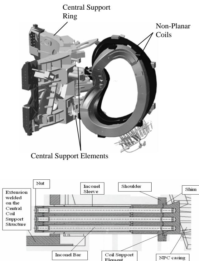
FIG. 2. NPC connected to the CSR, cross-section of a central support element bolted connection.
