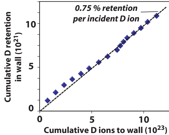
Fig. 5 Cumulative D retention in cleaned Mo walls versus incident D ion. Plasma conditions are as in Figs. 2 & 4.
