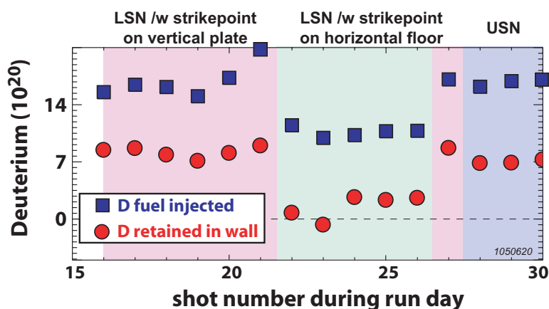
Fig. 3 Fuelled and retained D per shot with varying divertor magnetic geometries. LSN: lower single-null, USN: upper single-null. Experiment: boronized wall, I_p = 1 \text{ MA} , P_{ICRF} = 1 \text{ MW} , n_e \sim 1.6 \times 10^{20} \text{ m}^{-3} .
