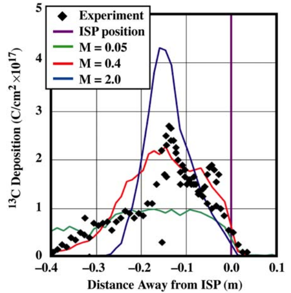
FIG. 8. OEDGE modeling of carbon flow shows a M \sim 0.4 agrees best with the L-mode data.
