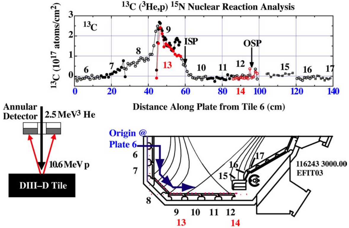
FIG. 3. Results from NRA analysis of DIII-D tiles exposed to L-mode plasmas, tiles not shown were below the detectability level of the measurement. The highest concentration is observed inboard of the ISP (detached divertor) in the lower divertor [5]. Naturally occurring ^{13}\text{C} has been subtracted.
