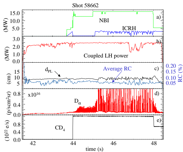
Figure 2. Time evolution of a) NBI and ICRH power, b) LH power, c) distance plasma-limiter in black and average RC in blue, d) D_\alpha signal and e) gas injection for shot 58662 with ( \text{CD}_4 )
