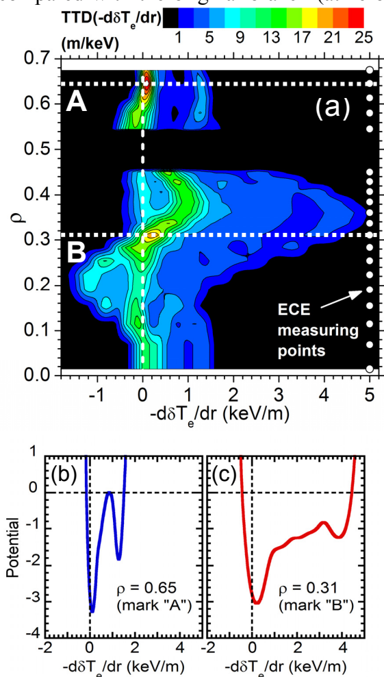
FIG. 5. (a) Contour plot of the transit time distribution (TTD) of the evaluated -\delta T_e/dr at 20-ECE measuring points for the plasma with the nonlocal transport phenomenon (LHD #49708). The ECE measuring points are indicated by white circles. Transport potential profiles, which are defined as -\ln(\text{TTD}) , (b) for \rho = 0.65 at mark “A” in (a) and (c) for \rho = 0.31 at mark “B” in (a).
