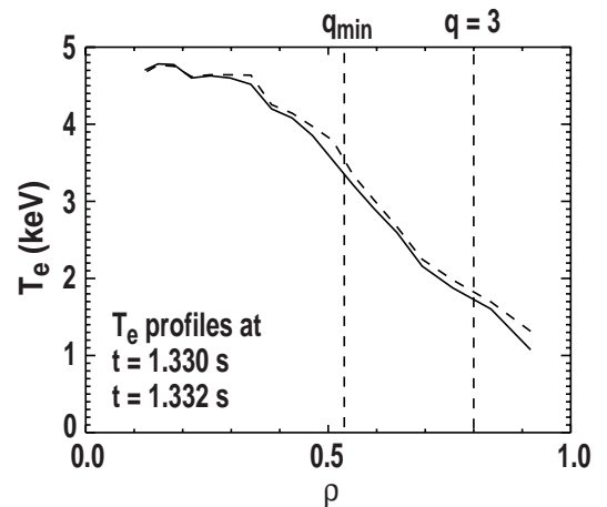
FIG. 2. Electron temperature profiles from electron cyclotron emission before (broken line) and during (solid line) the growth of a resistive wall mode (96519). Magnetic data indicates that the maximum inward displacement at the plasma edge is near the toroidal location of the ECE diagnostic.
