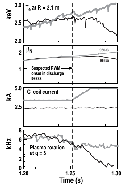
FIG. 4. Comparison of a discharge with a static n=1 perturbation applied to oppose the resistive wall mode (gray, upper curves, discharge 96633) and a discharge without the perturbation (solid, lower curves, discharge 96625). (a) Electron temperature near the q=3 surface. (b) Normalized beta. (c) C-coil current. (The non-zero dc level represents an n=3 bias field.) (d) Plasma rotation frequency at the q=3 surface.
