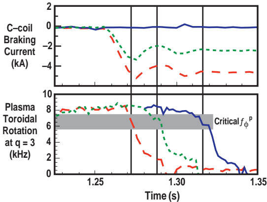
FIG. 3. Three discharges with varying amounts of magnetic braking (96514, 96518, 96515). (a) C-coil current applying an n=1 magnetic perturbation. (b) Plasma rotation frequency at the q=3 surface. The onset time of the resistive wall mode in each discharge is shown by a vertical line. The inferred critical rotation frequency is shown as a horizontal shaded band.
