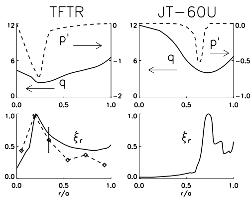
Figure 4: Plasma p and q profiles at the time of a BLM in TFTR and JT-60U and the r radial component of the displacement vector for an n = 1 pressure driven instability. The eigenvector of the instability is composed from a sum of several poloidal mode numbers which have different radial distributions. The mode number varies depending on the local- q value so that m \sim q_{\text{local}} . For example on JT-60U the mode number near the peak is m = 4 and near the plasma edge is m \sim 6 - 7 . An estimate of the experimental displacement, from the ECE data, is shown for TFTR. The maximum displacement is 5 mm.
