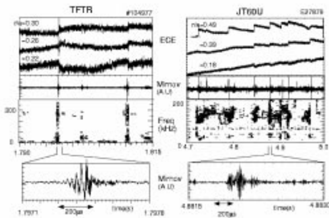
Figure 2: Traces of T_e and the Mirnov activity on TFTR and JT-60U showing the similar burst-like features of BLMs in both devices. Note the spatial localization and inversion in the T_e traces. The Mirnov activity coincides with the T_e bursts and the mode is seen to grow on a time scale shorter than 100\mu s .
