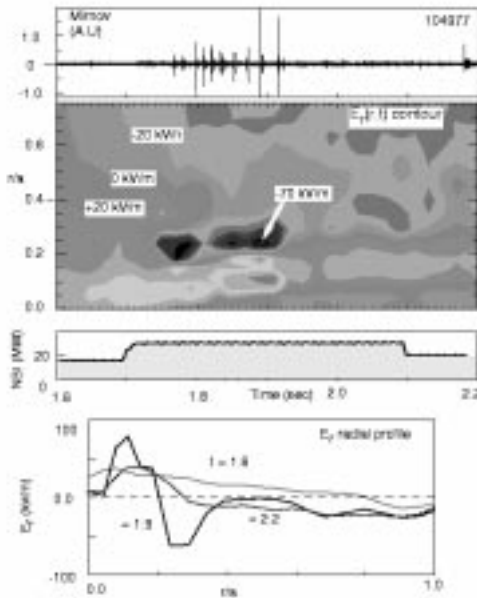
Figure 3: The BLM activity in TFTR sometimes coincides with intense negative radial electric fields. The top trace shows the Mirnov signal, the middle panel shows contours of the radial electric field which changes with time. The radial profile of E_r at times corresponding to the BLMs is shown in the lowest panel. Note that while the field shown here has a maximum negative value of 60\text{kV/m} ; in some bursts, field strengths in excess of 100\text{kV/m} have been observed.
