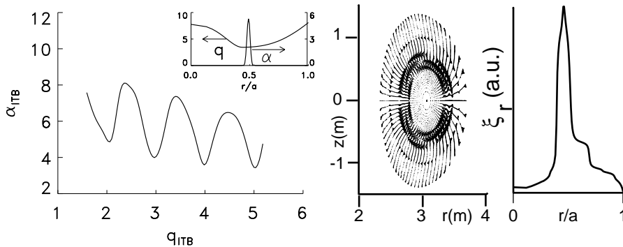
Figure 5: The stability limit of the n = 1 mode expressed in terms of the local pressure gradient and its dependence on the local- q value. An example of the model profiles used to determine this curve is shown in the inset. The dependence on q_{local} is determined by scaling the toroidal field. The mode structure of the instability is shown on the right hand side. The dominant poloidal mode number is m \sim q_{local} .
