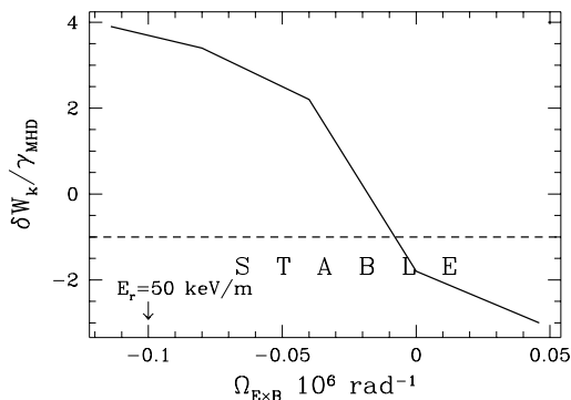
Figure 7: A strong negative electric field can kinetically destabilize an m > 1 internal mode.
