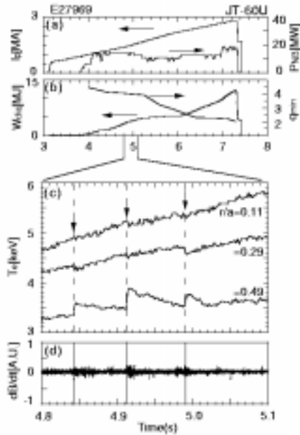
Figure 1: Time evolution of the (a) plasma current, I_p , neutral beam injection power P_{NB} , (b) stored energy, W_{dia} , and q_{min} on JT-60U for the length of the discharge. Panels (c) and (d) show an expanded view of a shorter time segment, where (c) has the evolution of T_e at three radii, and (d) shows the data from a Mirnov loop. Note the spatial localization and inversion in the T_e traces. The Mirnov activity coincides with the T_e bursts.
