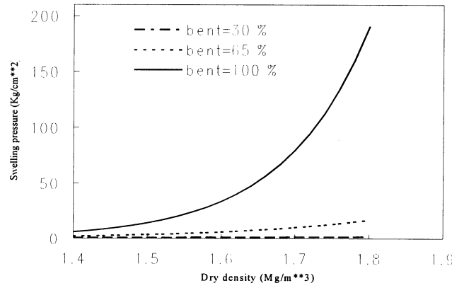
Fig. 2. Effect of dry density and bentonite content on the swelling pressure.
