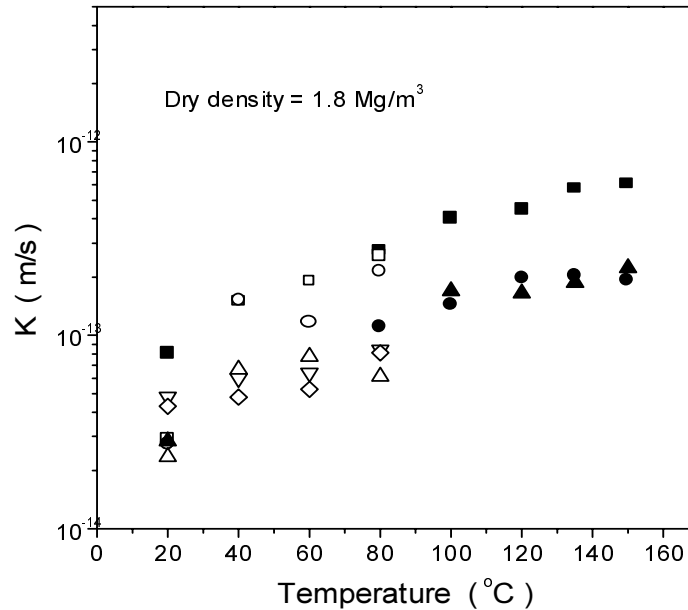
Fig.7. Influence of temperature elevation on the hydraulic conductivity of compacted bentonite.
