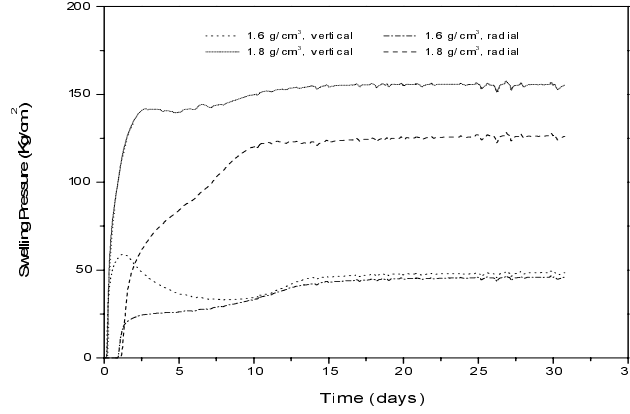
Fig. 1. Development of swelling pressure versus elapsed time for bentonite.
