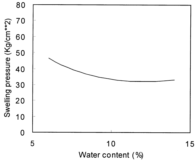
Fig.5. Effect of initial water content on the swelling pressure for bentonite (dry density=1.6 Mg/m 3 ).
