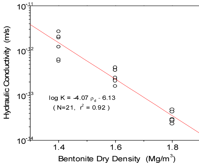
Fig.6. Hydraulic conductivity versus the dry density of compacted bentonite.
