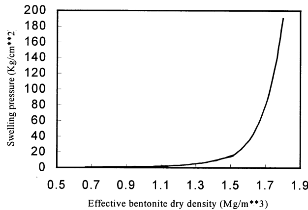
Fig.3. Swelling pressure as a function of effective clay dry density.
