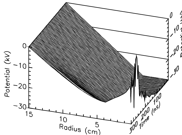
FIG. 4. Time behavior of potential profile
