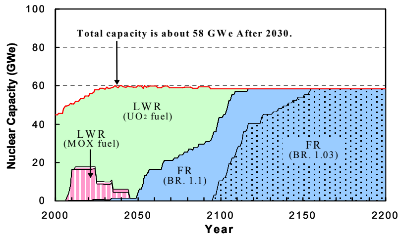
Figure 2.4. Transition scenario from LWR cycle to FR cycle in Japan.
