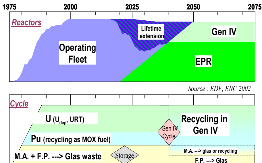
Figure 2.2. Evolution of the French nuclear reactors and fuel cycle technologies. (Gen IV = Generation IV reactors, U_{dep} = depleted uranium, U_{RT} = reprocessed uranium, M.A. = minor actinides, F.P. = fission products)
