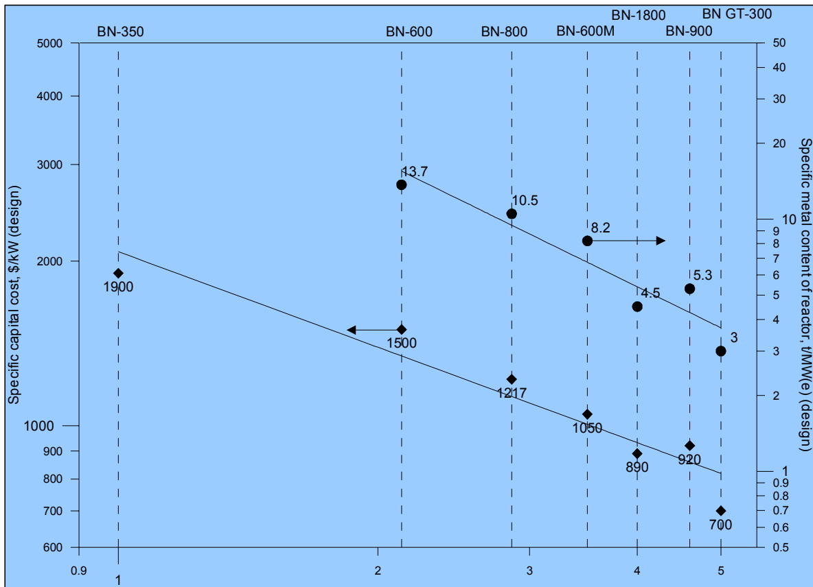
Figure 5.2. Reduction of capital cost of fast reactors due to R&D in Russia.
