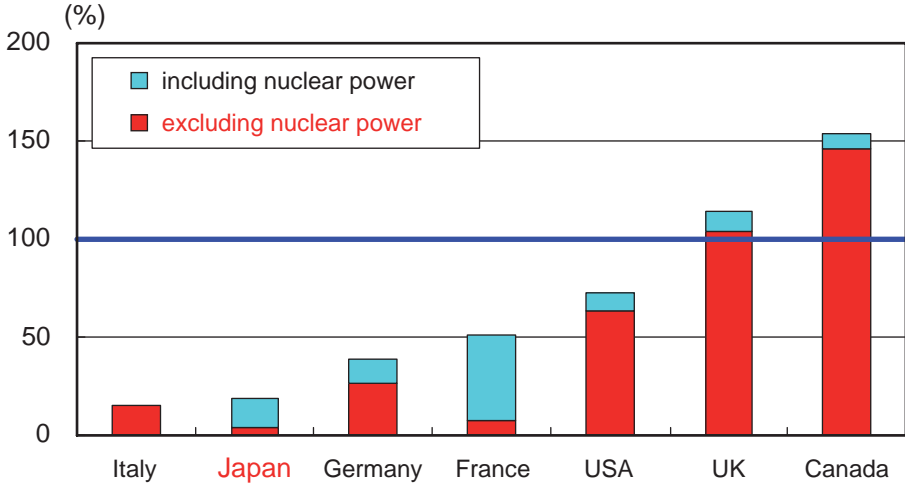
FIG. 3. Energy self-sufficiency of selected countries.
