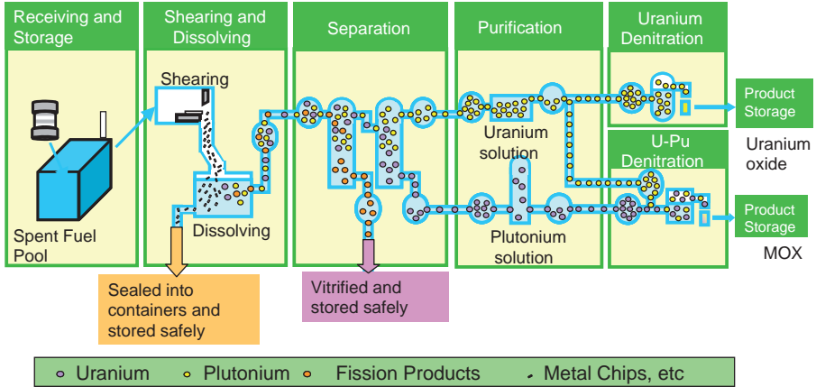
FIG. 6. Process used at the Rokkasho reprocessing plant.
