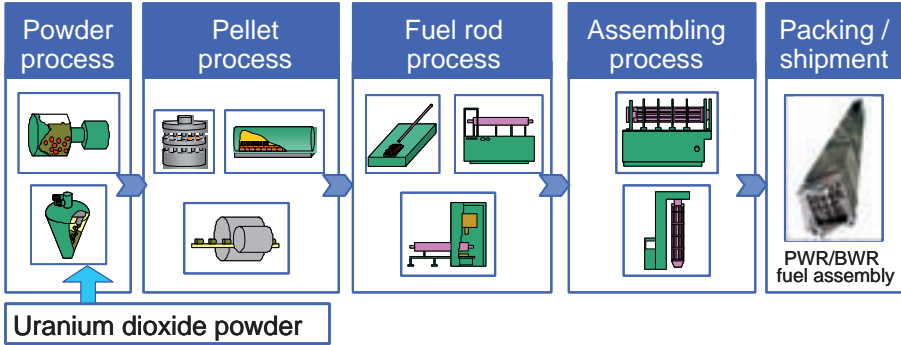
FIG. 8. Process outline of the JNFL MOX fuel plant.
