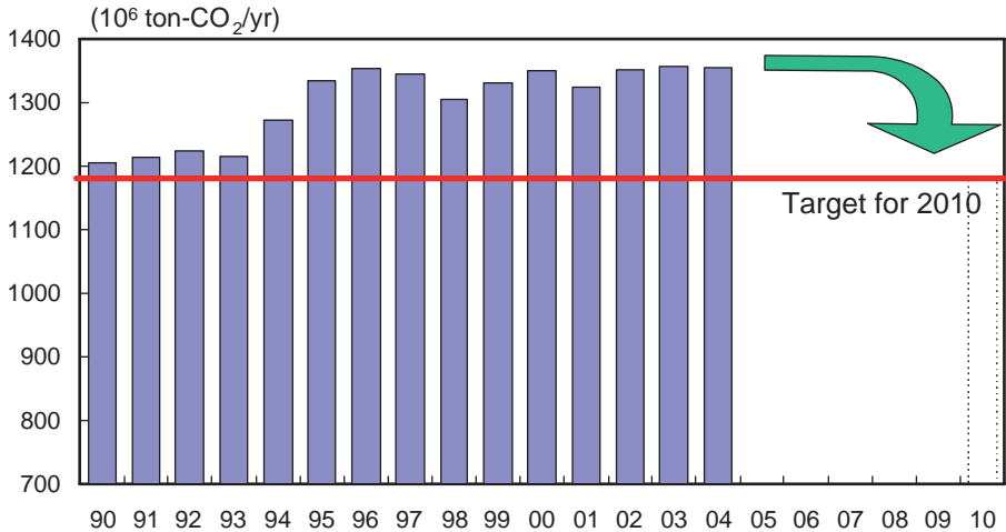
FIG. 4. Japan's Kyoto Protocol target for 2008–2012.
