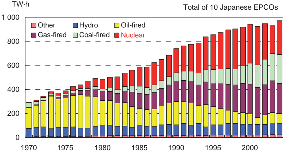
FIG. 1. Nuclear power generation since 1970.
