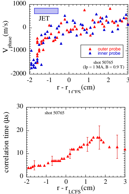
FIG. 2. Radial profiles of poloidal phase velocity of fluctuations and autocorrelation times in JET.
