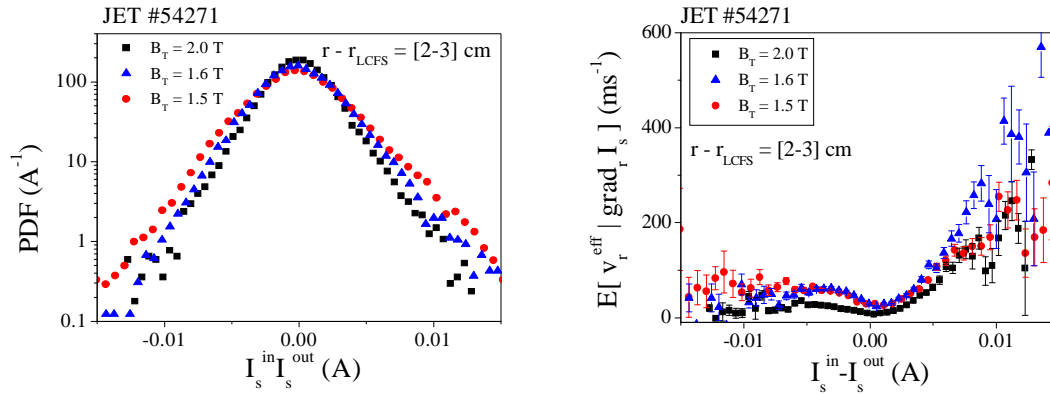
Fig. 8. PDFs of gradients and of effective radial velocities measured in the JET plasma boundary region.
