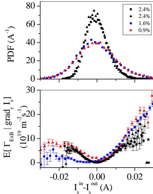
Fig. 7. PDFs of gradients and turbulent transport varying the magnetic well (0.9 – 2.4 %) in the TJ-II stellarator.
