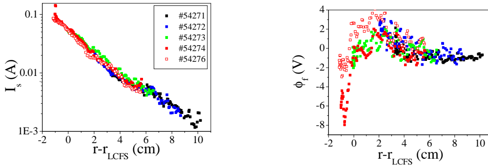
FIG. 3. Radial profiles of ion saturation current and floating potential in the JET boundary region (ohmic plasmas).
