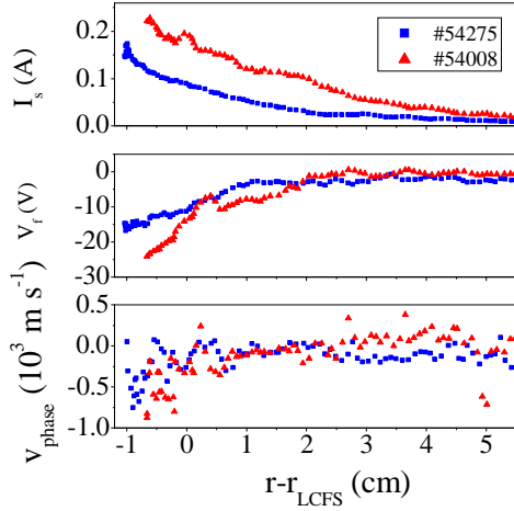
Fig. 5. Radial profiles in JET ohmic (shot 54275) and L-mode (shot 54008) plasmas.
