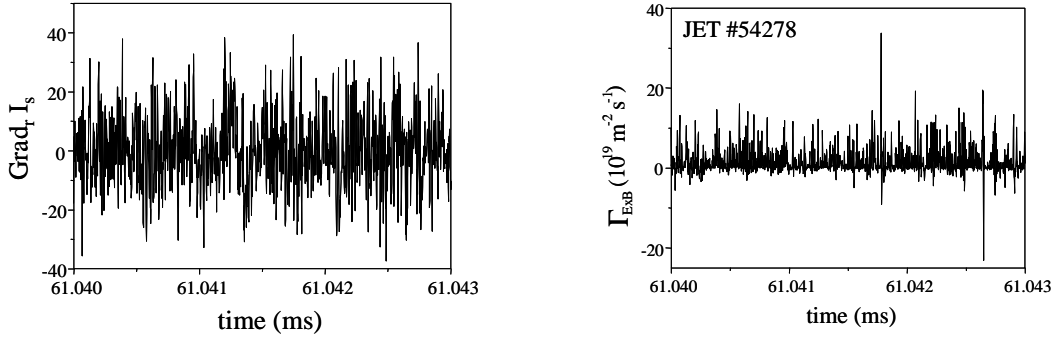
FIG. 1. Time evolution of the radial gradients and turbulent transport in the JET plasma boundary region.
