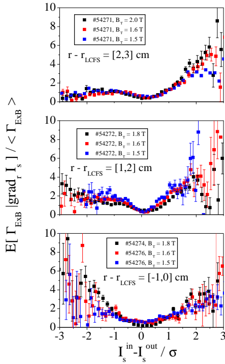
Fig. 4. Radial transport versus fluctuations in gradients in the JET boundary region.
