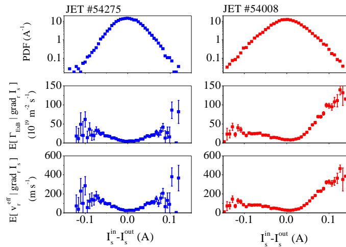
Fig. 6. PDFs of gradients, transport and radial effective velocity in ohmic (shot 54275) and L-mode plasmas (shot 54008) in the JET plasma boundary region.
