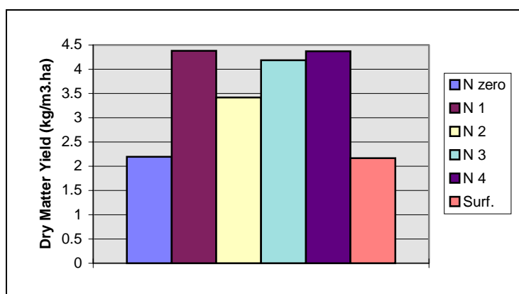
Fig. 3. Water use efficiency ( kg\ dry\ matter/m^3/ha ) of cotton under drip and surface irrigation.
