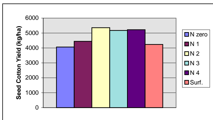
Fig. 2. Yield of seed-cotton for fertigation with 0, 60 (N1), 120 (N2), 180 (N3), and 240 (N4) kg N/ha and traditional surface irrigation with 180 kg N/ha (compare N3 and Surf.).
