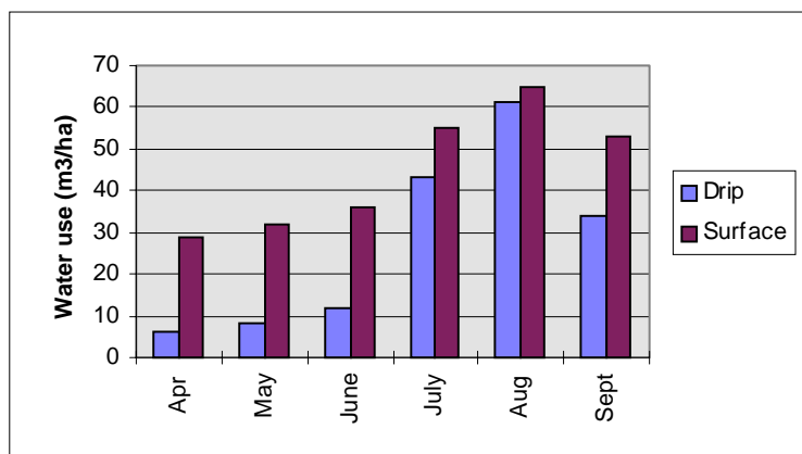
Fig. 1. Average daily evapo-transpiration ( m^3/ha ) during the growing season of cotton under drip and surface irrigation. Total water consumption was 4,900 m^3/ha (drip) and 7,600 m^3/ha (surface).
