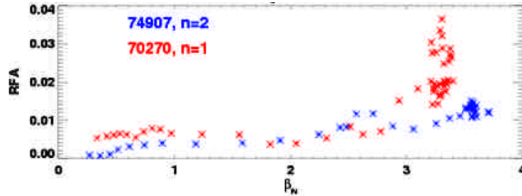
FIG.7. n = 1 and n = 2 probing in similar pulses.
