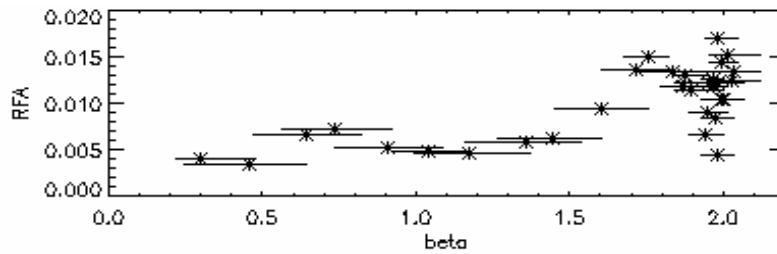
FIG.8. Non-monotonic n=2 RFA response observed prior to the 1 st ELM at low \beta_N below the RFA threshold, #75862.
