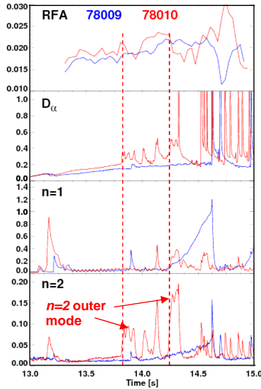
FIG.6. Reduction in RFA observed during the outer mode. From top to bottom: RFA, D_\alpha , n=1 and n=2 mode amplitude. Blue – #78009, no outer mode, red – #78010, with outer mode.
