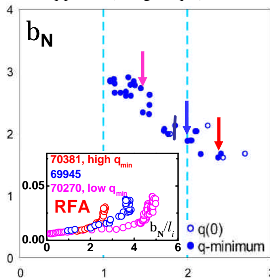
FIG.2. Decrease in RFA threshold measured in the high- b_N low or slightly reversed shear pulses with q_{\min} determined using EFIT constrained by MSE, polarimetry, pressure, low- n MHD and Alfvén Cascades. Inset: Sudden increase in the RFA, indicating the no-wall limit, does not correlate (at different q_{\min} ) with integral parameters (e.g. 4l_i )
