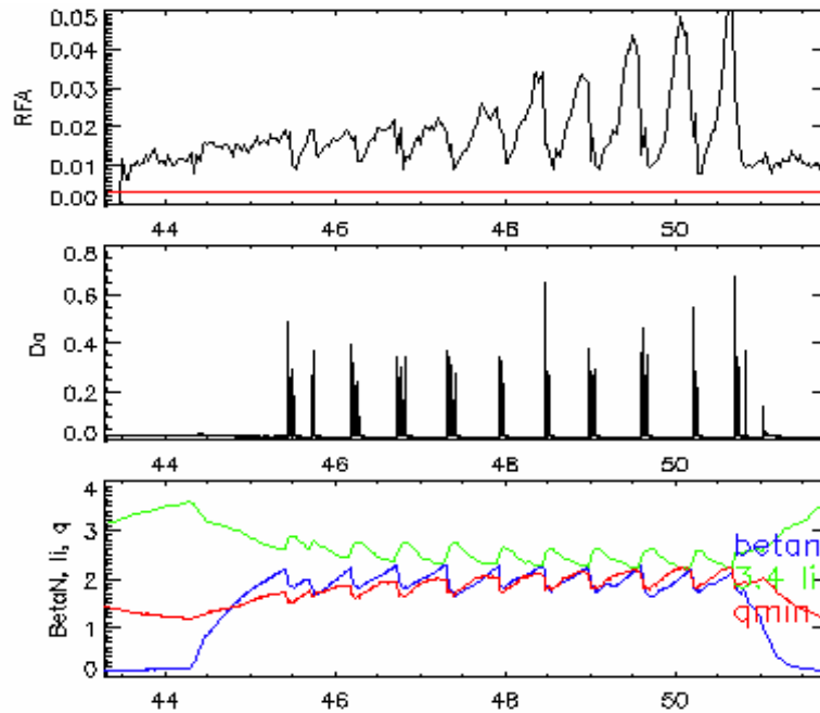
FIG.4. RFA (top) increases during ELM-free periods (middle), at constant low b_N and marginal evolution of other integral parameters (bottom plot), #73092. (Plasma pulse starts at t=40 s in this and the next figures).
