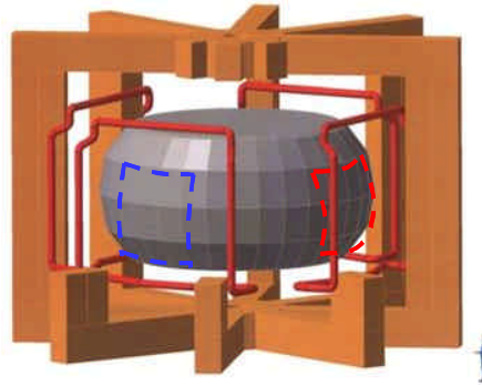
FIG.1. Position of the external Error Field Correction Coils (solid red) and measuring loops (dashed red and blue, only 2 of 4 saddle loops are shown) on JET.
