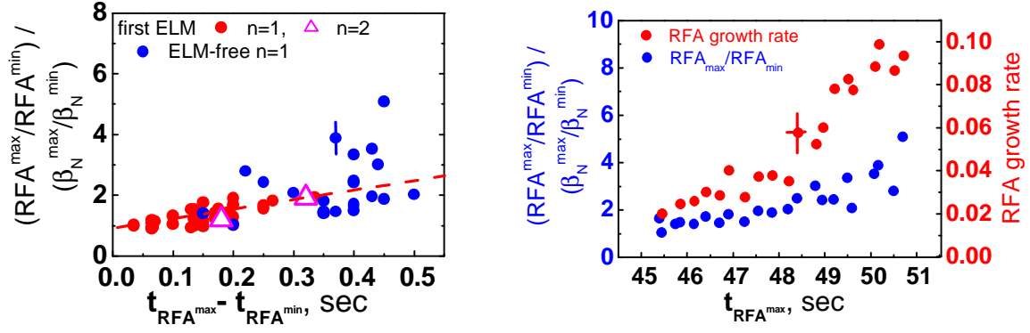
FIG.5. Left: RFA growth vs growth time during ELM-free period before 1 st ELM, \bullet n=1 , \triangle n=2 and during ELM-free periods at flat-top in ##73091,92, \bullet n=1 . Red line shows linear fit to the data before 1 st ELM. Right: RFA growth and RFA growth rate vs time (at RFA_{max} ) in ##73091, 92 during pulse flat-top.
