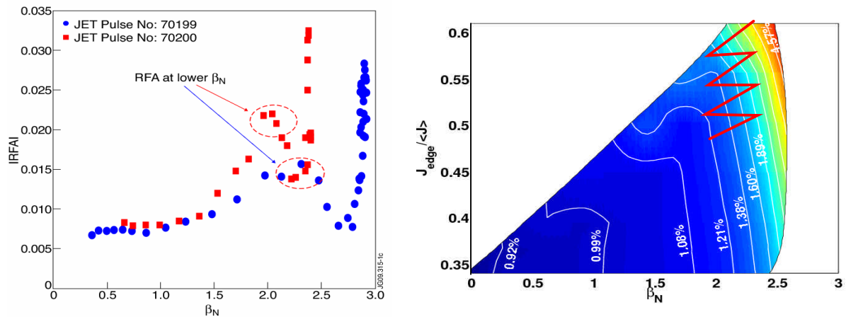
FIG.3. Non-monotonic n=1 RFA response observed at low \beta_N well below the RFA threshold, prior to the 1 st ELM, left, and the simulated RFA response (white contours, in %), MARS-F, right. Red zigzag line shows cartoon of a possible edge current evolution, as discussed in Section 3.
