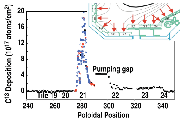
FIG. 6. ^{13}\text{C} density as a function of position for injection into the lower divertor (2008) of a LSN plasma. The second thermo-oxidation experiment used this same configuration for deposition and tiles were removed for analysis.
