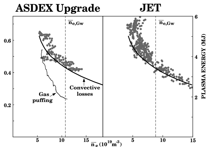
FIG. 6: Plasma energy versus line averaged density reached with steady state pellet injection (filled circles). Solid curves: expected confinement reduction caused by pellet added convective losses. Operational area limitation for gas puff refuelling in ASDEX Upgrade is also given for comparison.
