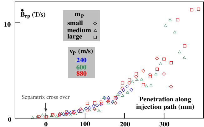
FIG. 2: Pellet induced MHD perturbation in AUG versus pellet position along the injection path, separatrix position defines 0. At the same position in the plasma, the same magnitude for the pellet driven MHD response is observed for any pellet speed and/or mass applied.
