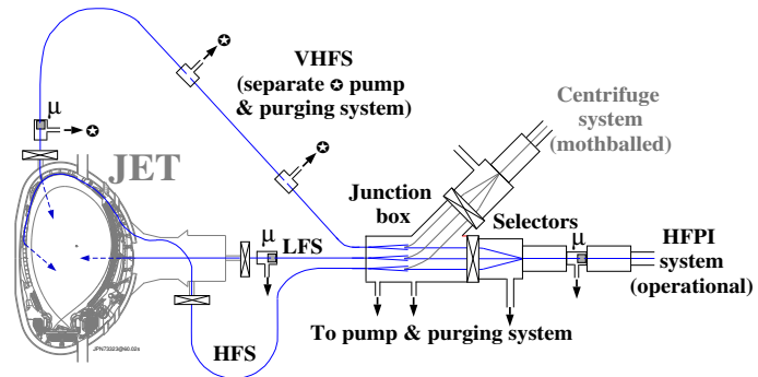
FIG. 1: The JET multi-injector multi-track pellet launching system under commissioning and put into operation during the experimental campaigns in 2008. With the new injector (HFPI) it is capable to perform both ELM pacing and fuelling experiments with high relevance to ITER. The available pellet size and velocity operational regime in combination with three injection tracks at different poloidal locations provides potential for dedicated physics experiments with respect to fuelling and ELM control physics.
