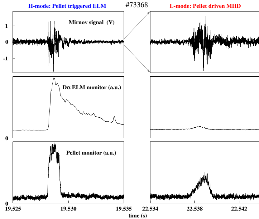
FIG. 4: Mirnov coil response, divertor D_\alpha ELM monitor and pellet ablation (top to bottom) for pellets in JET (accompanied possibly by debris) triggering an ELM during an H-mode phase (left) but driving only transient MHD activity declining after burn out (right, note expanded y-scale of upper box).
