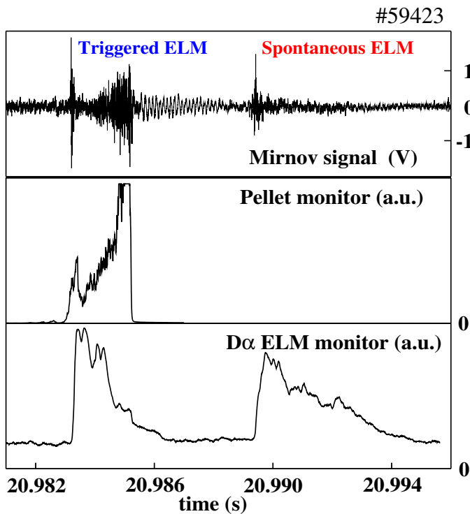
FIG. 3: Mirnov coil response, pellet ablation and divertor D_\alpha ELM monitor (top to bottom) for a fuelling size ( 4 \times 10^{21} D) pellet triggered (left) and a spontaneous (right) ELM in JET.
