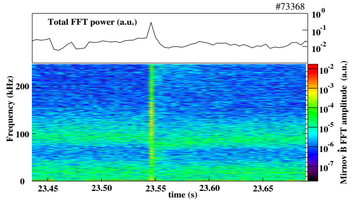
FIG. 5: Mirnov coil signal frequency amplitude evolution before, during and after pellet injection into a JET L-mode phase (lower) and according integrated amplitude (upper). The pellet causes a transient short directly driven strong increase of the mode amplitude and a longer lasting drop in the frequency attributed to fuelling.
